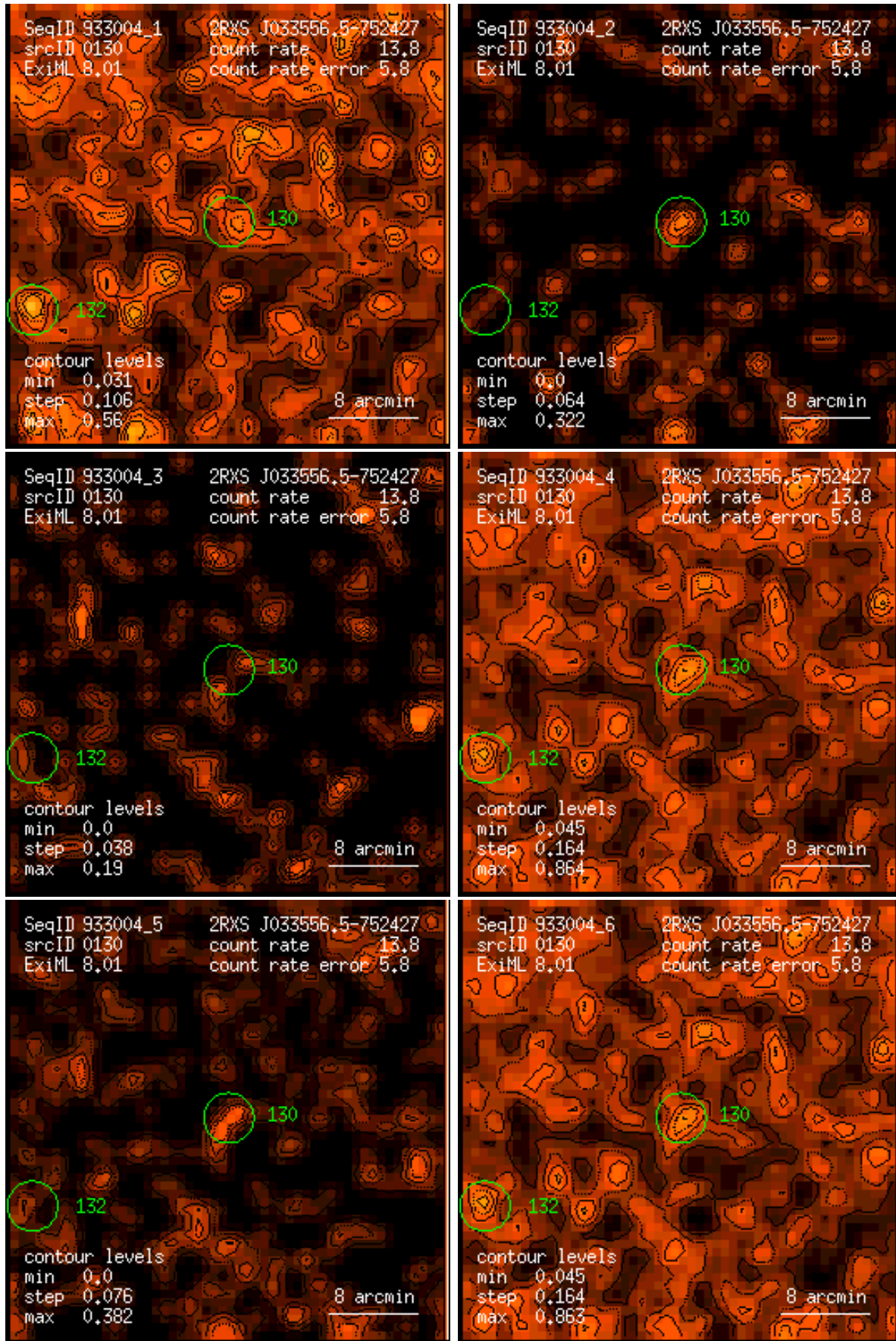
Figure 130: RASS 933004: detection 0130: band rate images, Gaussian filter: (1) PSPC channels 11 – 41, (2) 52 – 90, (3) 91 – 201, (4) 11 – 235, (5) 52 – 201, (6) 11 – 201. Broad band rates in counts/ks. Band rate contour levels in counts/ks/arcmin 2 .
