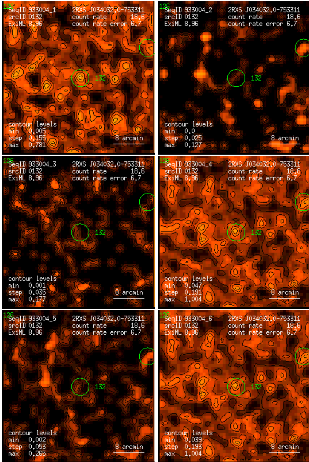
Figure 132: RASS 933004: detection 0132: band rate images, Gaussian filter: (1) PSPC channels 11 – 41, (2) 52 – 90, (3) 91 – 201, (4) 11 – 235, (5) 52 – 201, (6) 11 – 201. Broad band rates in counts/ks. Band rate contour levels in counts/ks/arcmin 2 .
