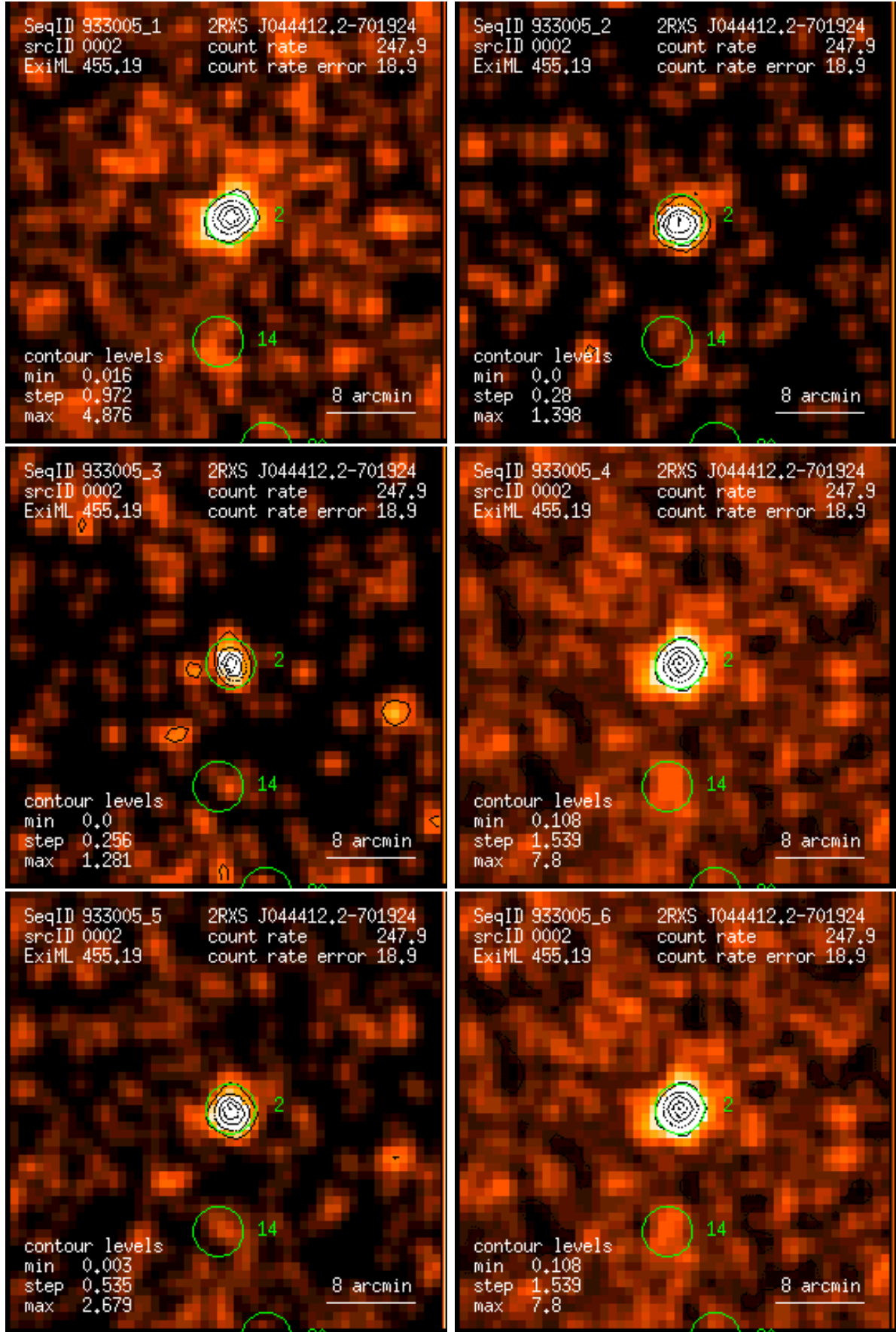
Figure 2: RASS 933005: detection 0002: band rate images, Gaussian filter: (1) PSPC channels 11 – 41, (2) 52 – 90, (3) 91 – 201, (4) 11 – 235, (5) 52 – 201, (6) 11 – 201. Broad band rates in counts/ks. Band rate contour levels in counts/ks/arcmin 2 .
