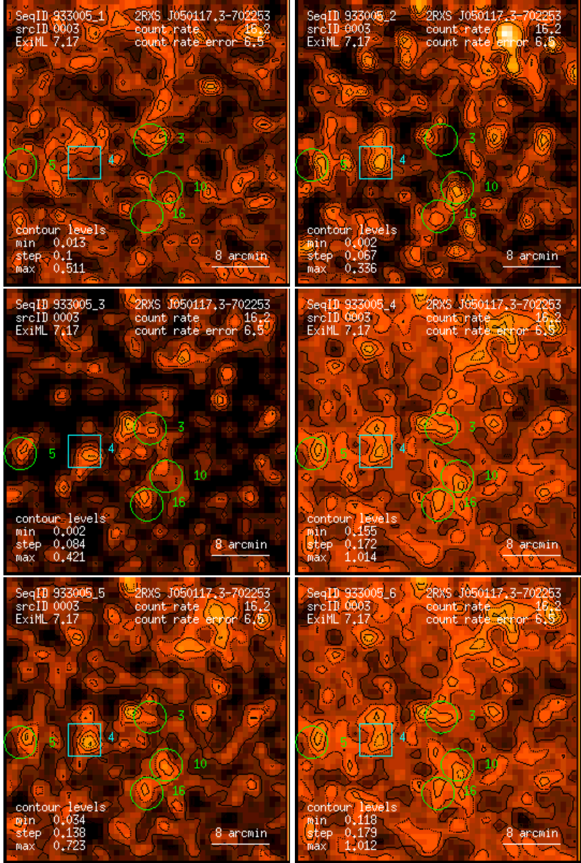
Figure 3: RASS 933005: detection 0003: band rate images, Gaussian filter: (1) PSPC channels 11 – 41, (2) 52 – 90, (3) 91 – 201, (4) 11 – 235, (5) 52 – 201, (6) 11 – 201. Broad band rates in counts/ks. Band rate contour levels in counts/ks/arcmin 2 .
