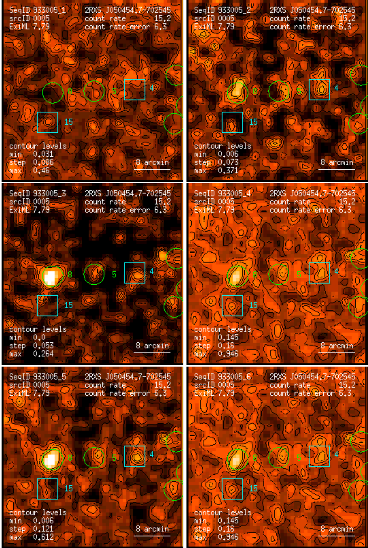
Figure 5: RASS 933005: detection 0005: band rate images, Gaussian filter: (1) PSPC channels 11 – 41, (2) 52 – 90, (3) 91 – 201, (4) 11 – 235, (5) 52 – 201, (6) 11 – 201. Broad band rates in counts/ks. Band rate contour levels in counts/ks/arcmin 2 .
