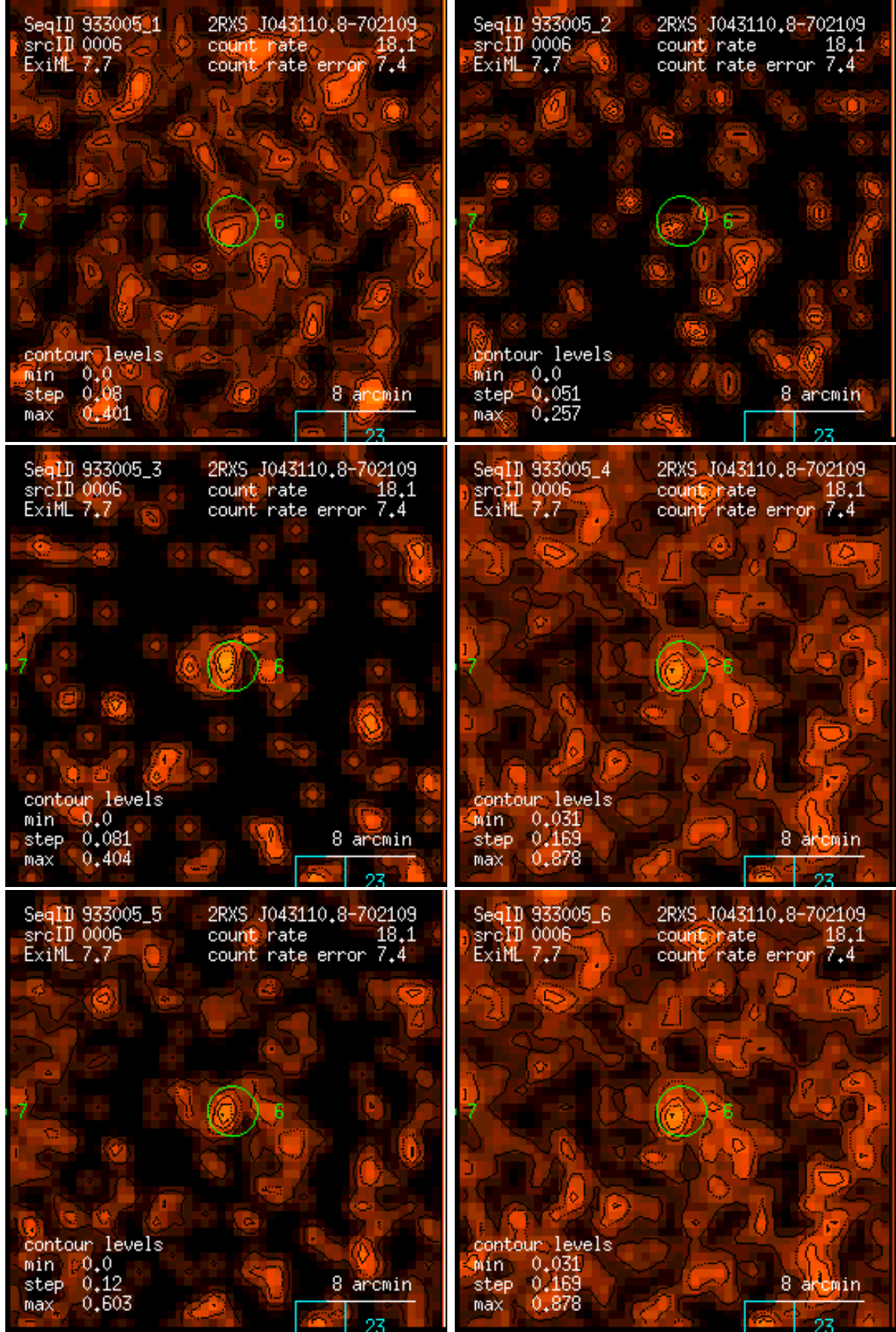
Figure 6: RASS 933005: detection 0006: band rate images, Gaussian filter: (1) PSPC channels 11 – 41, (2) 52 – 90, (3) 91 – 201, (4) 11 – 235, (5) 52 – 201, (6) 11 – 201. Broad band rates in counts/ks. Band rate contour levels in counts/ks/arcmin 2 .
