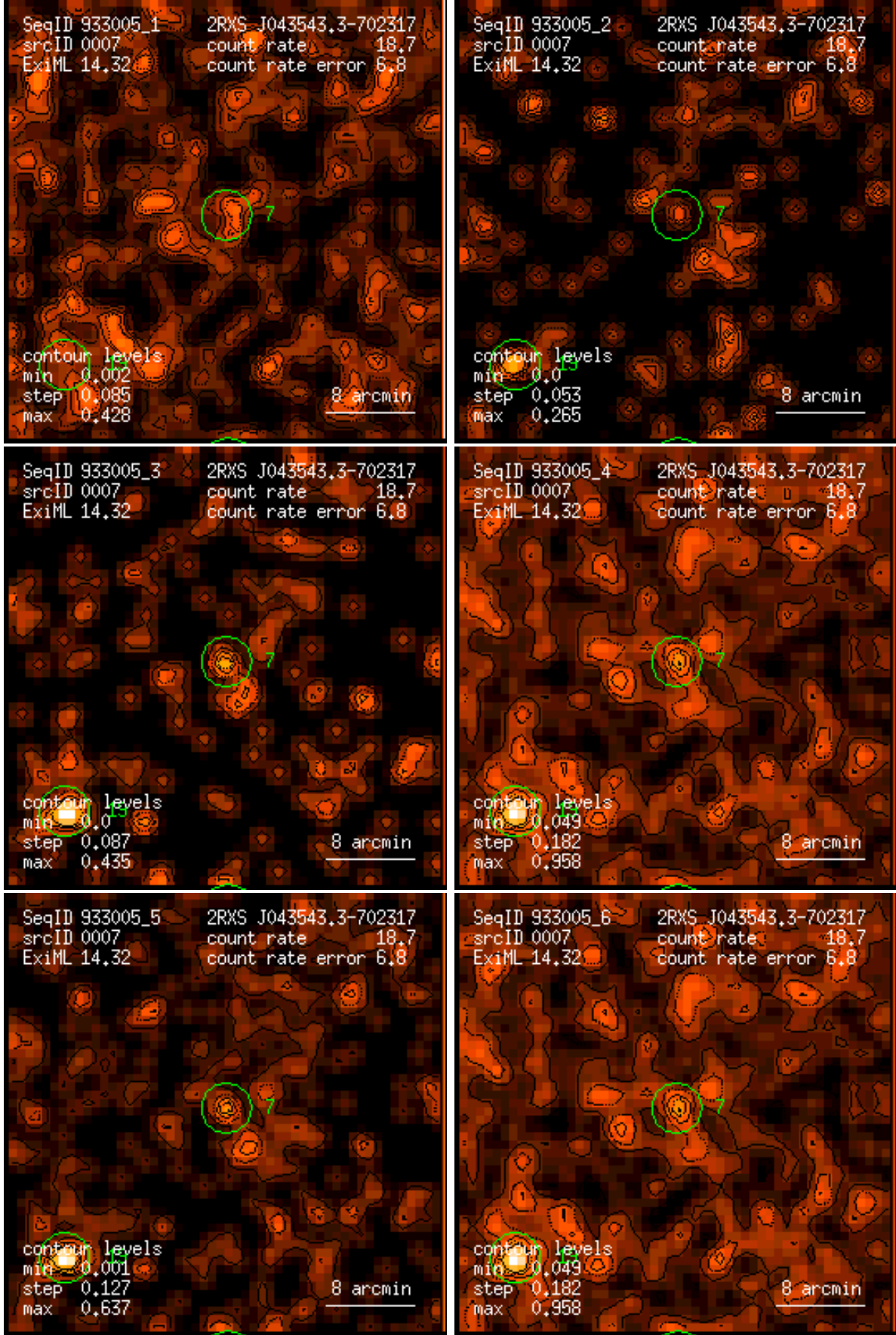
Figure 7: RASS 933005: detection 0007: band rate images, Gaussian filter: (1) PSPC channels 11 – 41, (2) 52 – 90, (3) 91 – 201, (4) 11 – 235, (5) 52 – 201, (6) 11 – 201. Broad band rates in counts/ks. Band rate contour levels in counts/ks/arcmin 2 .
