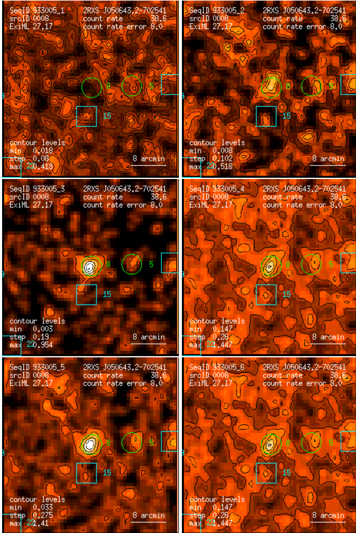
Figure 8: RASS 933005: detection 0008: band rate images, Gaussian filter: (1) PSPC channels 11 – 41, (2) 52 – 90, (3) 91 – 201, (4) 11 – 235, (5) 52 – 201, (6) 11 – 201. Broad band rates in counts/ks. Band rate contour levels in counts/ks/arcmin 2 .
