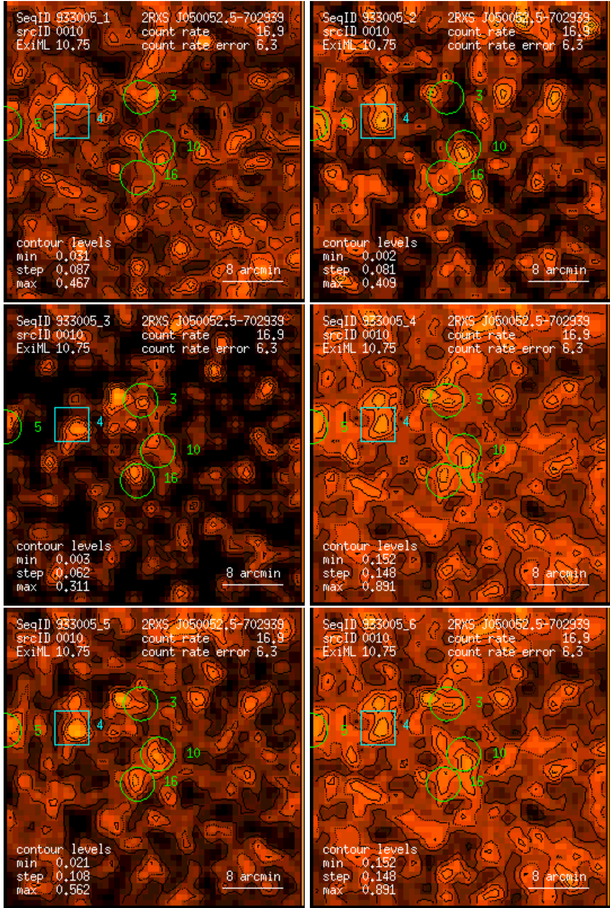
Figure 10: RASS 933005: detection 0010: band rate images, Gaussian filter: (1) PSPC channels 11 – 41, (2) 52 – 90, (3) 91 – 201, (4) 11 – 235, (5) 52 – 201, (6) 11 – 201. Broad band rates in counts/ks. Band rate contour levels in counts/ks/arcmin 2 .
