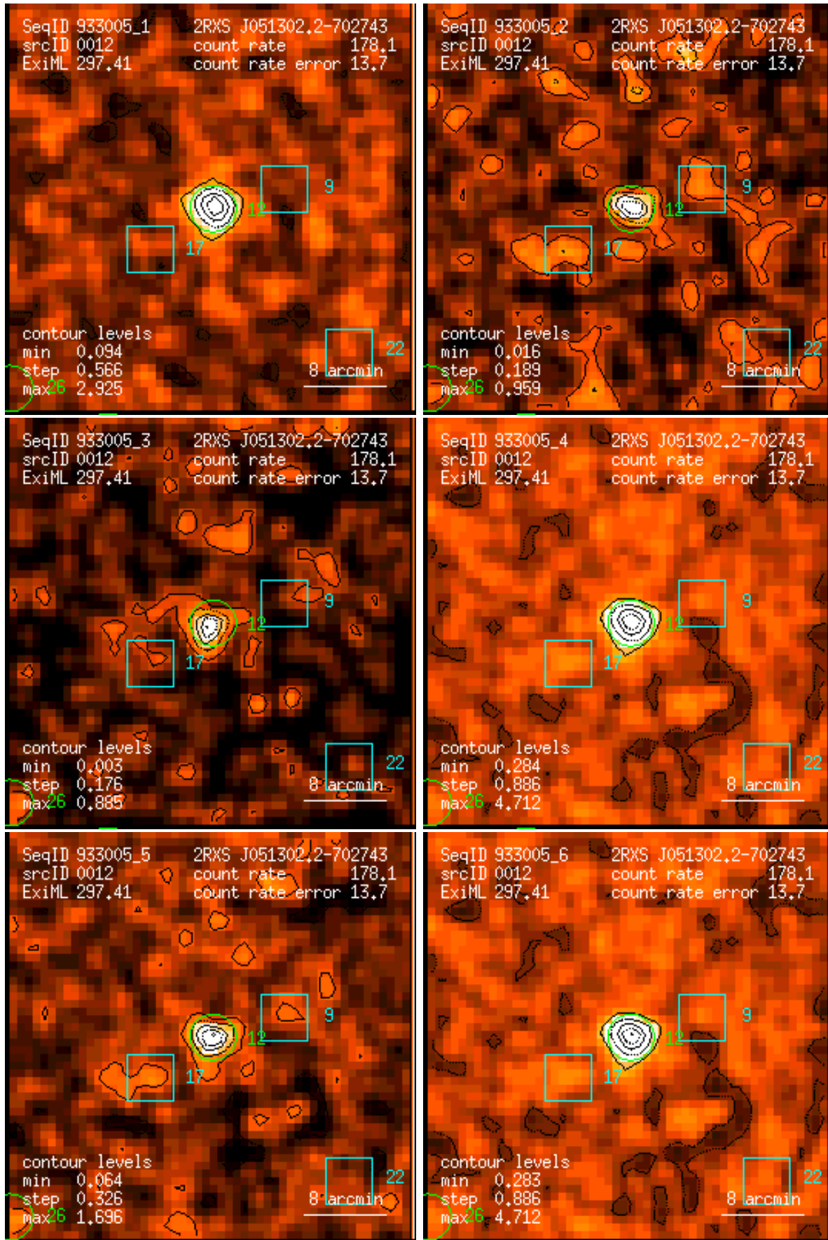
Figure 12: RASS 933005: detection 0012: band rate images, Gaussian filter: (1) PSPC channels 11 – 41, (2) 52 – 90, (3) 91 – 201, (4) 11 – 235, (5) 52 – 201, (6) 11 – 201. Broad band rates in counts/ks. Band rate contour levels in counts/ks/arcmin 2 .
