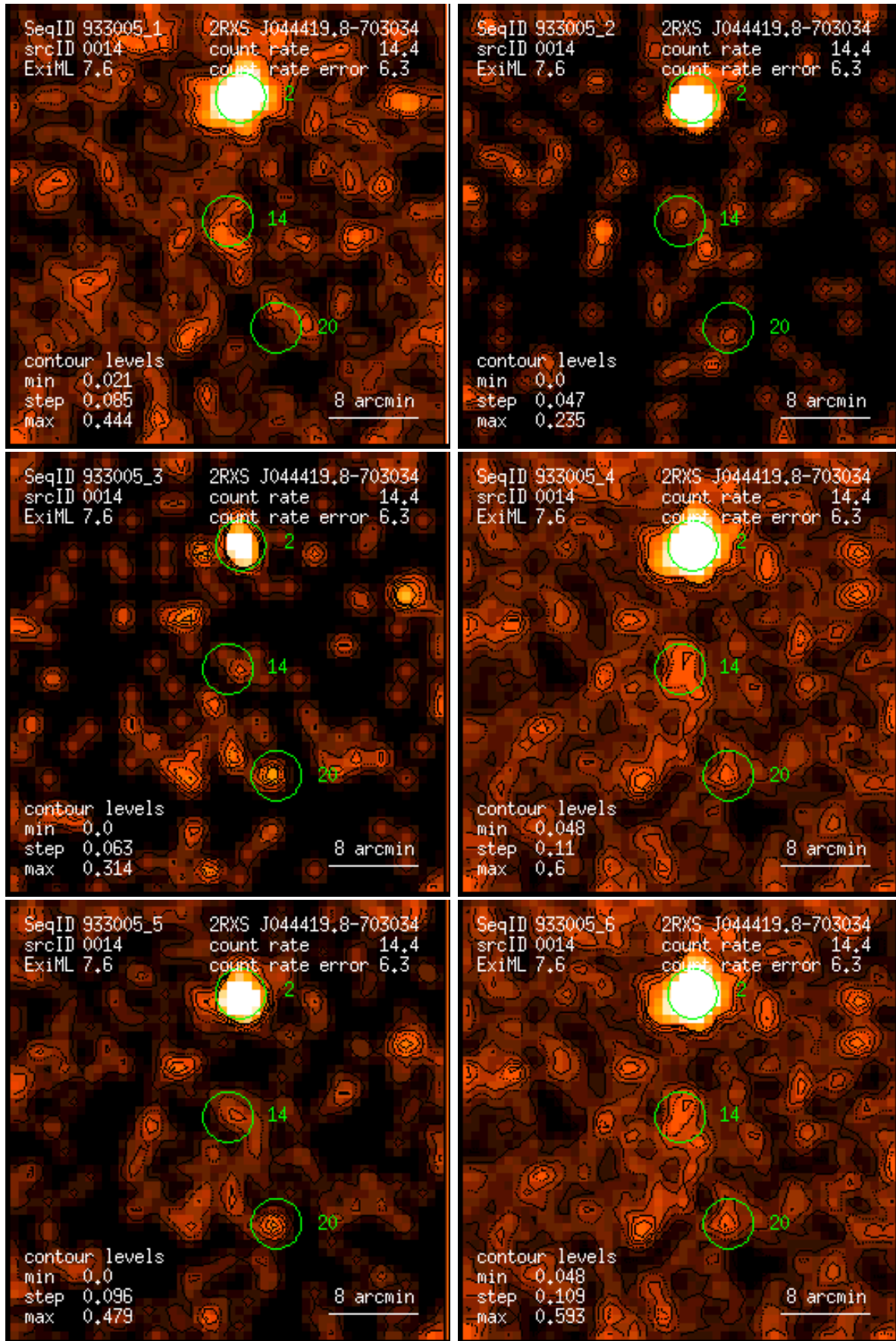
Figure 14: RASS 933005: detection 0014: band rate images, Gaussian filter: (1) PSPC channels 11 – 41, (2) 52 – 90, (3) 91 – 201, (4) 11 – 235, (5) 52 – 201, (6) 11 – 201. Broad band rates in counts/ks. Band rate contour levels in counts/ks/arcmin 2 .
