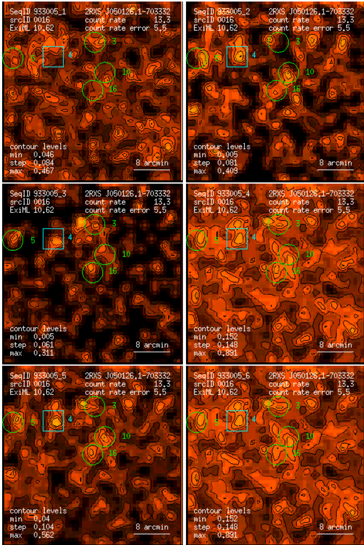
Figure 16: RASS 933005: detection 0016: band rate images, Gaussian filter: (1) PSPC channels 11 – 41, (2) 52 – 90, (3) 91 – 201, (4) 11 – 235, (5) 52 – 201, (6) 11 – 201. Broad band rates in counts/ks. Band rate contour levels in counts/ks/arcmin 2 .
