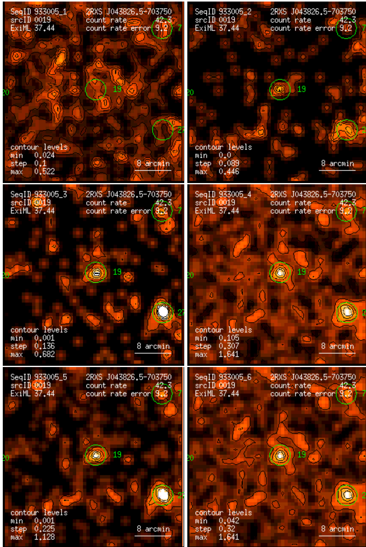
Figure 19: RASS 933005: detection 0019: band rate images, Gaussian filter: (1) PSPC channels 11 – 41, (2) 52 – 90, (3) 91 – 201, (4) 11 – 235, (5) 52 – 201, (6) 11 – 201. Broad band rates in counts/ks. Band rate contour levels in counts/ks/arcmin 2 .
