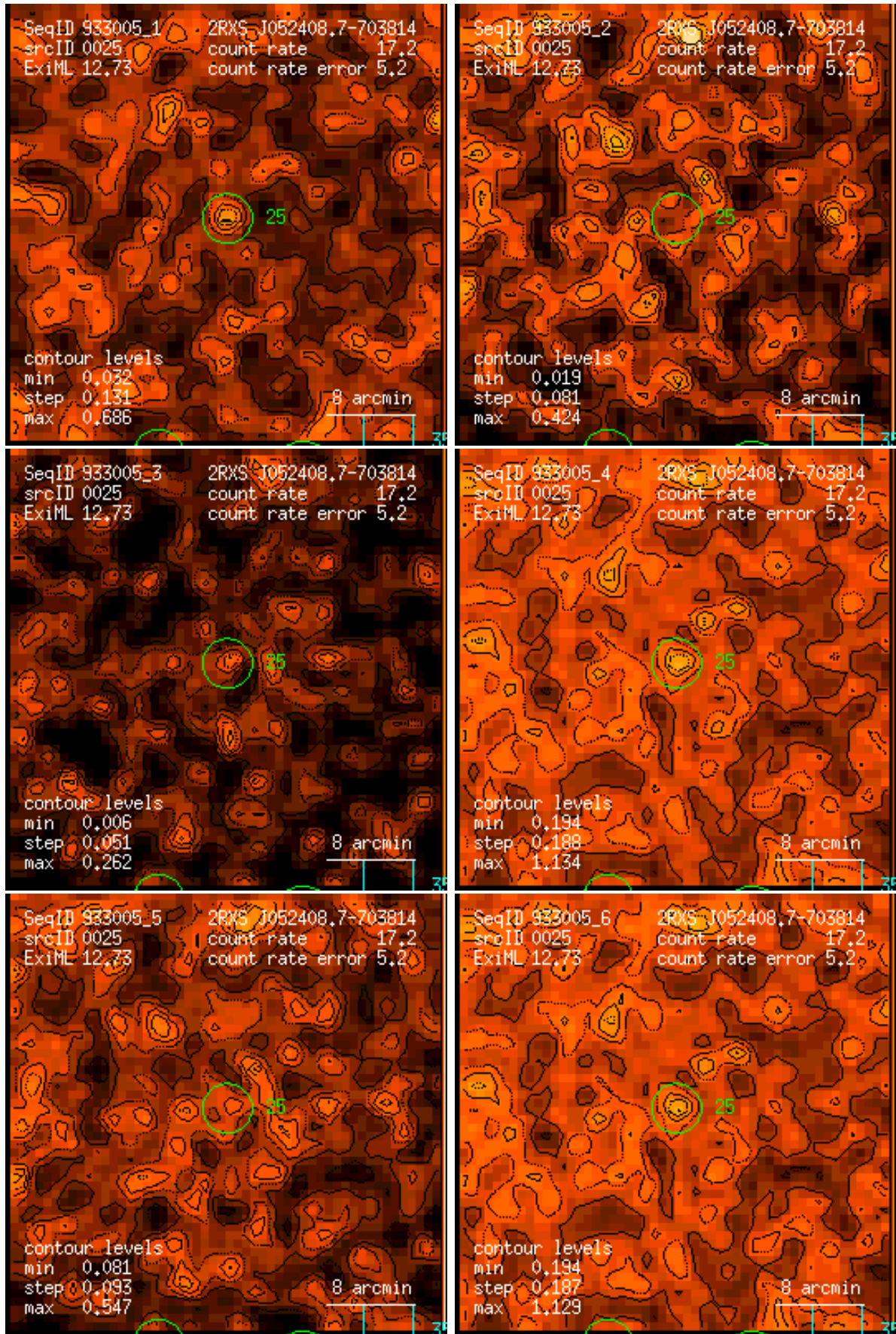
Figure 25: RASS 933005: detection 0025: band rate images, Gaussian filter: (1) PSPC channels 11 – 41, (2) 52 – 90, (3) 91 – 201, (4) 11 – 235, (5) 52 – 201, (6) 11 – 201. Broad band rates in counts/ks. Band rate contour levels in counts/ks/arcmin 2 .
