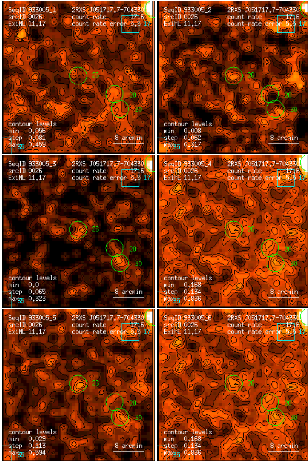
Figure 26: RASS 933005: detection 0026: band rate images, Gaussian filter: (1) PSPC channels 11 – 41, (2) 52 – 90, (3) 91 – 201, (4) 11 – 235, (5) 52 – 201, (6) 11 – 201. Broad band rates in counts/ks. Band rate contour levels in counts/ks/arcmin 2 .
