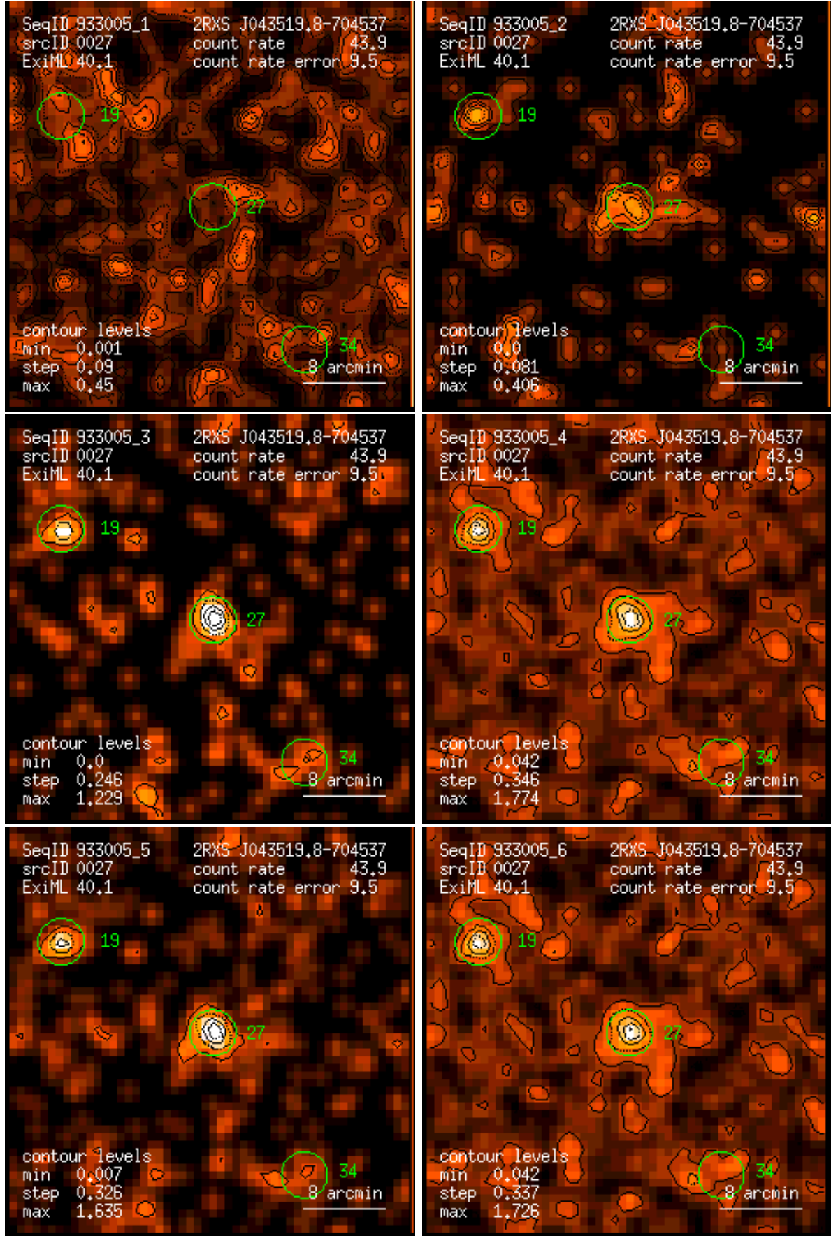
Figure 27: RASS 933005: detection 0027: band rate images, Gaussian filter: (1) PSPC channels 11 – 41, (2) 52 – 90, (3) 91 – 201, (4) 11 – 235, (5) 52 – 201, (6) 11 – 201. Broad band rates in counts/ks. Band rate contour levels in counts/ks/arcmin 2 .
