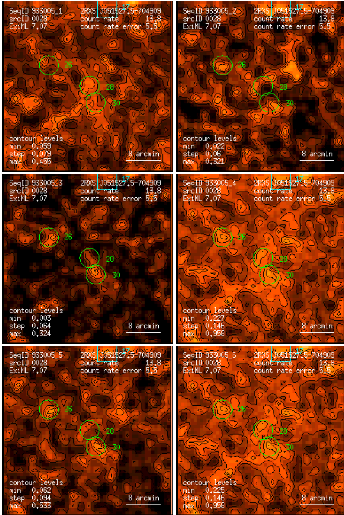
Figure 28: RASS 933005: detection 0028: band rate images, Gaussian filter: (1) PSPC channels 11 – 41, (2) 52 – 90, (3) 91 – 201, (4) 11 – 235, (5) 52 – 201, (6) 11 – 201. Broad band rates in counts/ks. Band rate contour levels in counts/ks/arcmin 2 .
