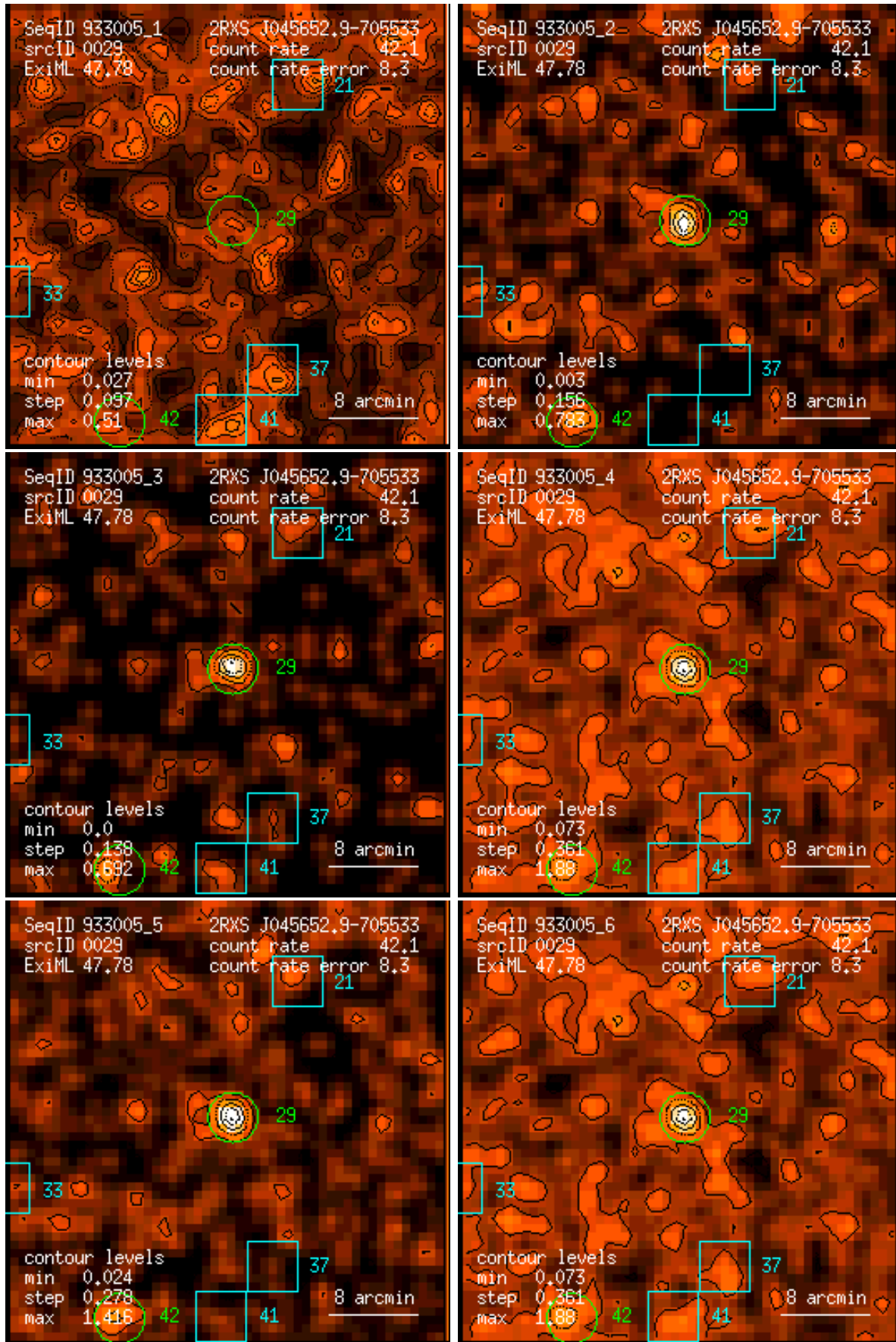
Figure 29: RASS 933005: detection 0029: band rate images, Gaussian filter: (1) PSPC channels 11 – 41, (2) 52 – 90, (3) 91 – 201, (4) 11 – 235, (5) 52 – 201, (6) 11 – 201. Broad band rates in counts/ks. Band rate contour levels in counts/ks/arcmin 2 .
