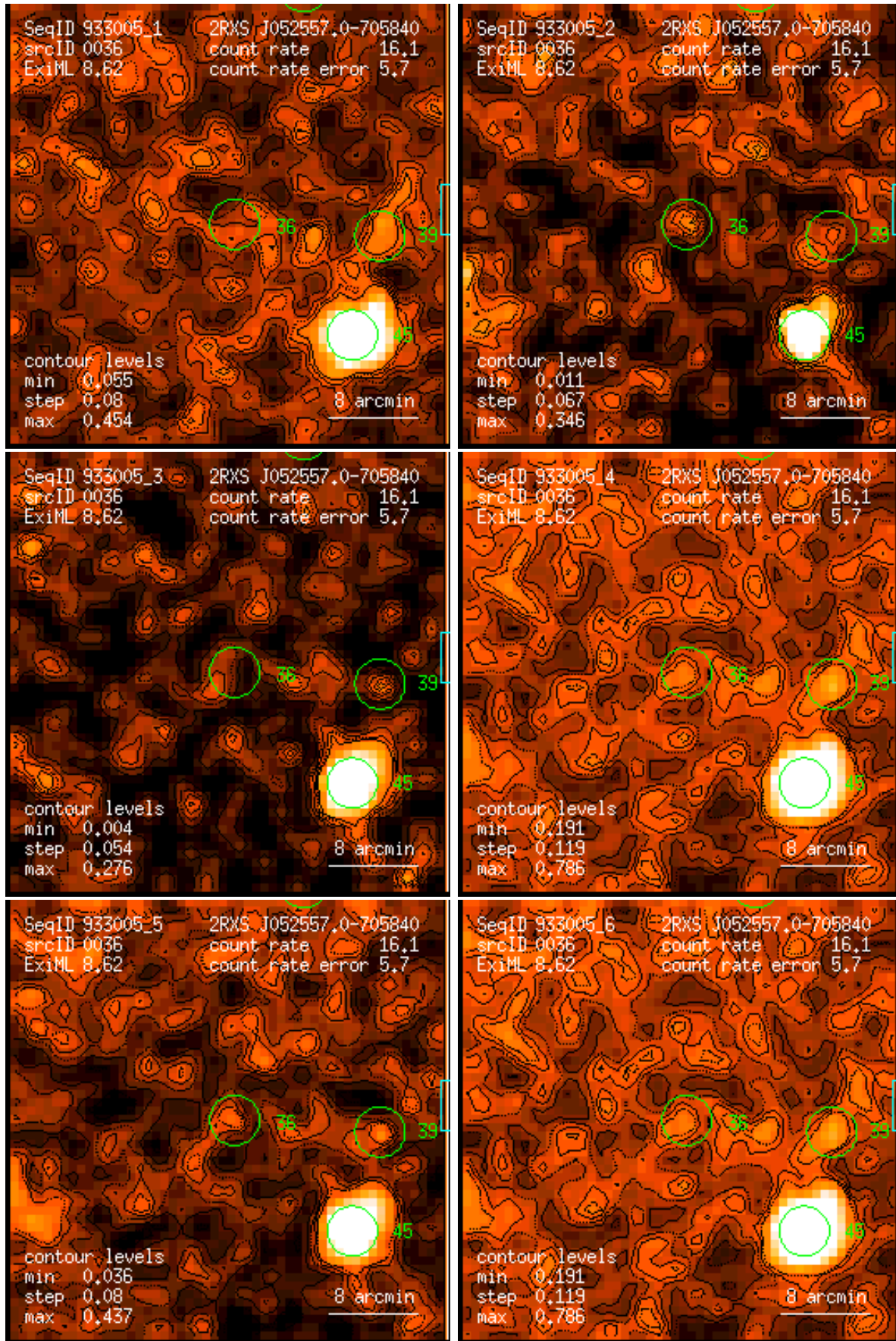
Figure 36: RASS 933005: detection 0036: band rate images, Gaussian filter: (1) PSPC channels 11 – 41, (2) 52 – 90, (3) 91 – 201, (4) 11 – 235, (5) 52 – 201, (6) 11 – 201. Broad band rates in counts/ks. Band rate contour levels in counts/ks/arcmin 2 .
