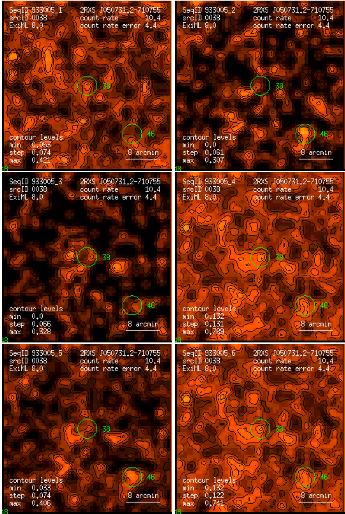
Figure 38: RASS 933005: detection 0038: band rate images, Gaussian filter: (1) PSPC channels 11 – 41, (2) 52 – 90, (3) 91 – 201, (4) 11 – 235, (5) 52 – 201, (6) 11 – 201. Broad band rates in counts/ks. Band rate contour levels in counts/ks/arcmin 2 .
