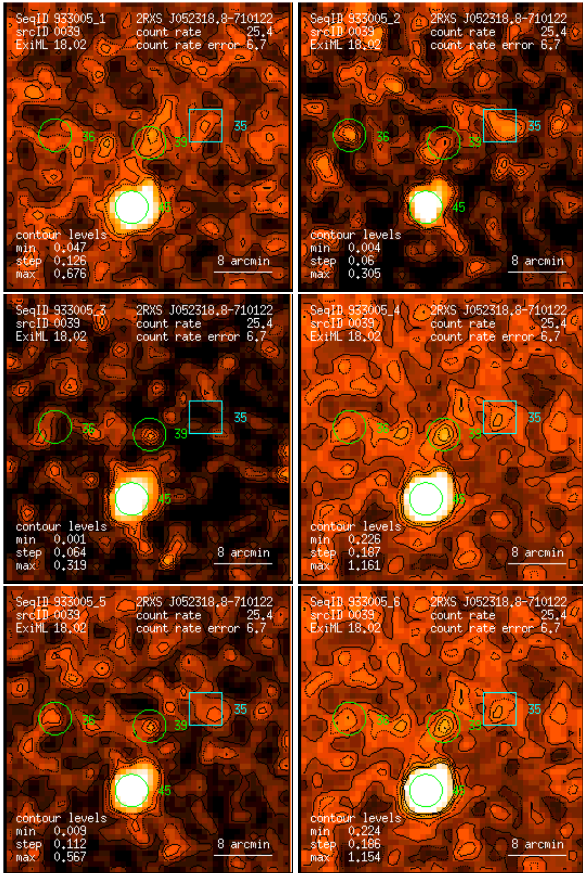
Figure 39: RASS 933005: detection 0039: band rate images, Gaussian filter: (1) PSPC channels 11 – 41, (2) 52 – 90, (3) 91 – 201, (4) 11 – 235, (5) 52 – 201, (6) 11 – 201. Broad band rates in counts/ks. Band rate contour levels in counts/ks/arcmin 2 .
