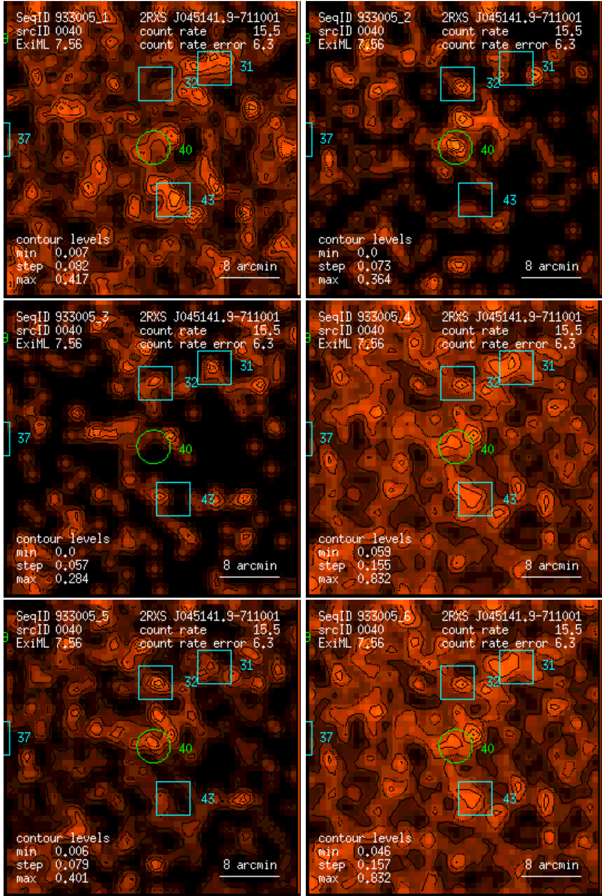
Figure 40: RASS 933005: detection 0040: band rate images, Gaussian filter: (1) PSPC channels 11 – 41, (2) 52 – 90, (3) 91 – 201, (4) 11 – 235, (5) 52 – 201, (6) 11 – 201. Broad band rates in counts/ks. Band rate contour levels in counts/ks/arcmin 2 .
