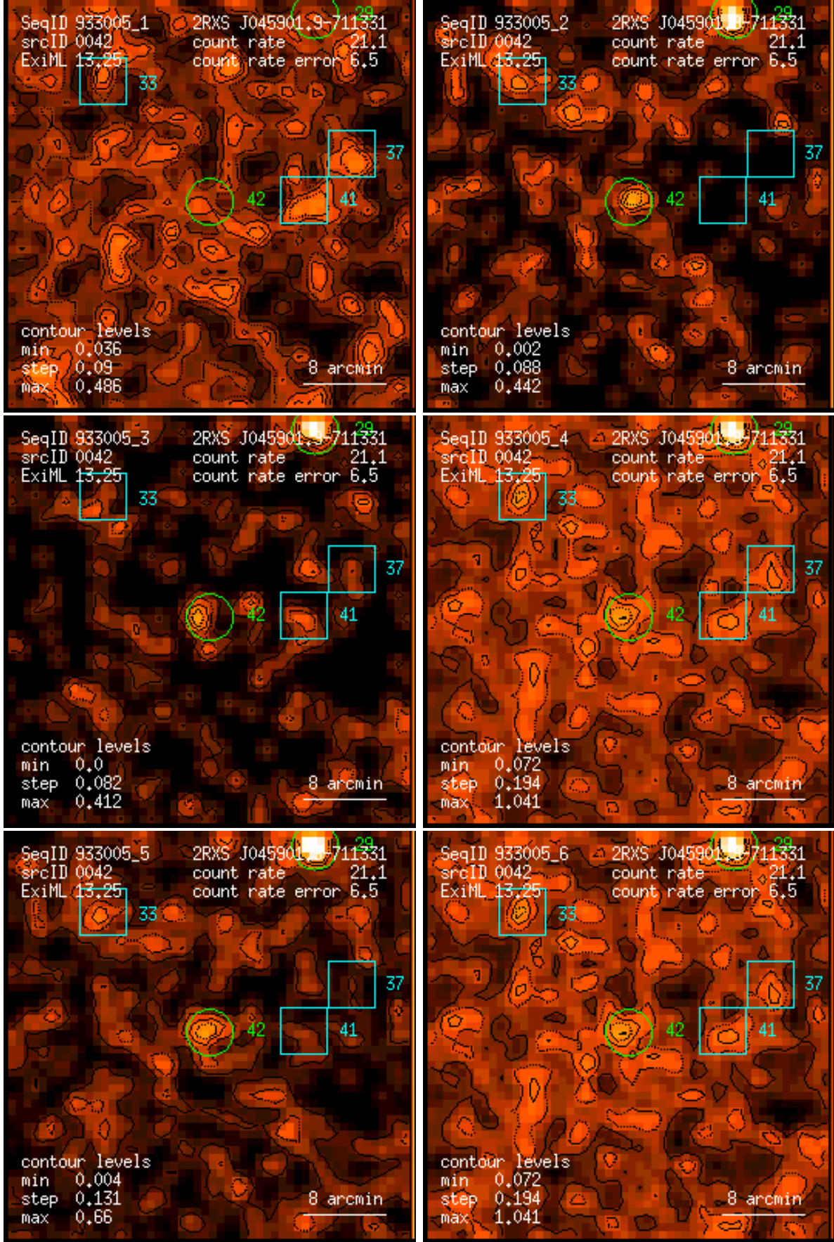
Figure 42: RASS 933005: detection 0042: band rate images, Gaussian filter: (1) PSPC channels 11 – 41, (2) 52 – 90, (3) 91 – 201, (4) 11 – 235, (5) 52 – 201, (6) 11 – 201. Broad band rates in counts/ks. Band rate contour levels in counts/ks/arcmin 2 .
