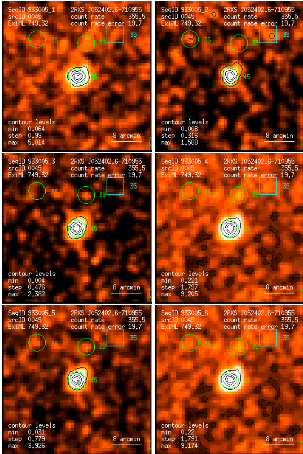
Figure 45: RASS 933005: detection 0045: band rate images, Gaussian filter: (1) PSPC channels 11 – 41, (2) 52 – 90, (3) 91 – 201, (4) 11 – 235, (5) 52 – 201, (6) 11 – 201. Broad band rates in counts/ks. Band rate contour levels in counts/ks/arcmin 2 .
