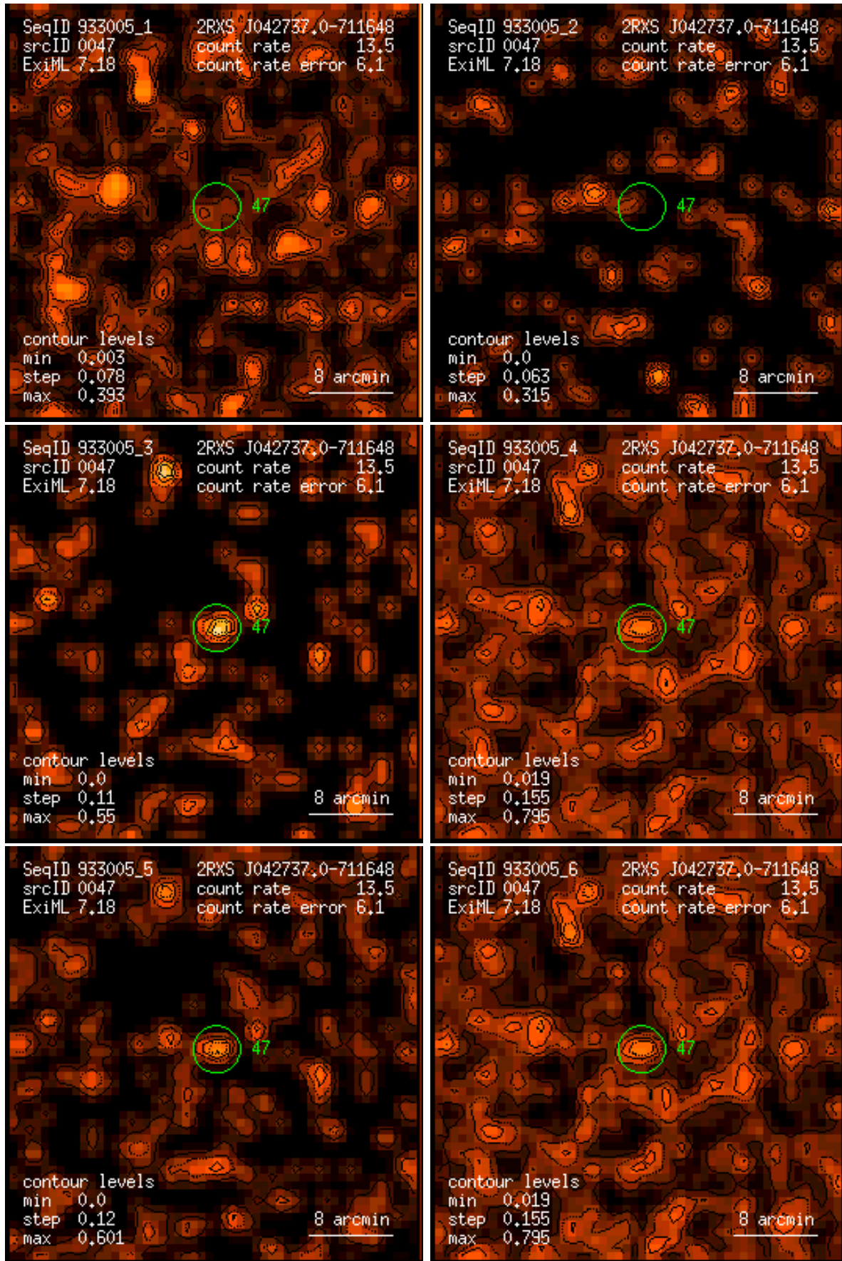
Figure 47: RASS 933005: detection 0047: band rate images, Gaussian filter: (1) PSPC channels 11 – 41, (2) 52 – 90, (3) 91 – 201, (4) 11 – 235, (5) 52 – 201, (6) 11 – 201. Broad band rates in counts/ks. Band rate contour levels in counts/ks/arcmin 2 .
