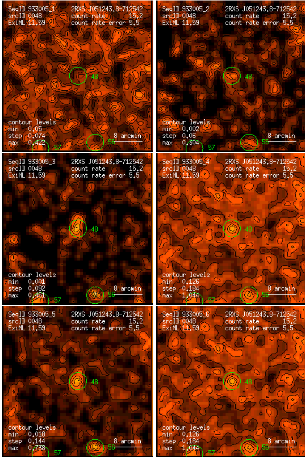
Figure 48: RASS 933005: detection 0048: band rate images, Gaussian filter: (1) PSPC channels 11 – 41, (2) 52 – 90, (3) 91 – 201, (4) 11 – 235, (5) 52 – 201, (6) 11 – 201. Broad band rates in counts/ks. Band rate contour levels in counts/ks/arcmin 2 .
