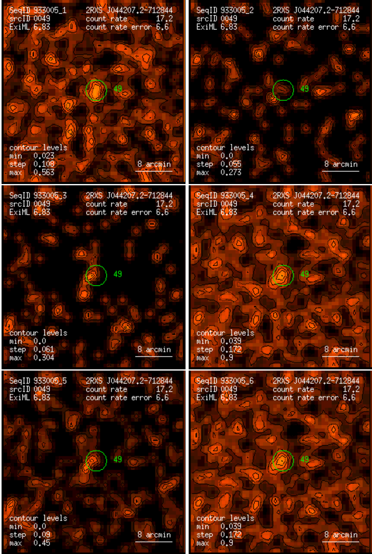
Figure 49: RASS 933005: detection 0049: band rate images, Gaussian filter: (1) PSPC channels 11 – 41, (2) 52 – 90, (3) 91 – 201, (4) 11 – 235, (5) 52 – 201, (6) 11 – 201. Broad band rates in counts/ks. Band rate contour levels in counts/ks/arcmin 2 .
