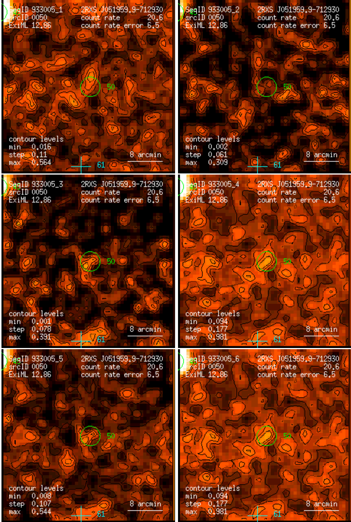
Figure 50: RASS 933005: detection 0050: band rate images, Gaussian filter: (1) PSPC channels 11 – 41, (2) 52 – 90, (3) 91 – 201, (4) 11 – 235, (5) 52 – 201, (6) 11 – 201. Broad band rates in counts/ks. Band rate contour levels in counts/ks/arcmin 2 .
