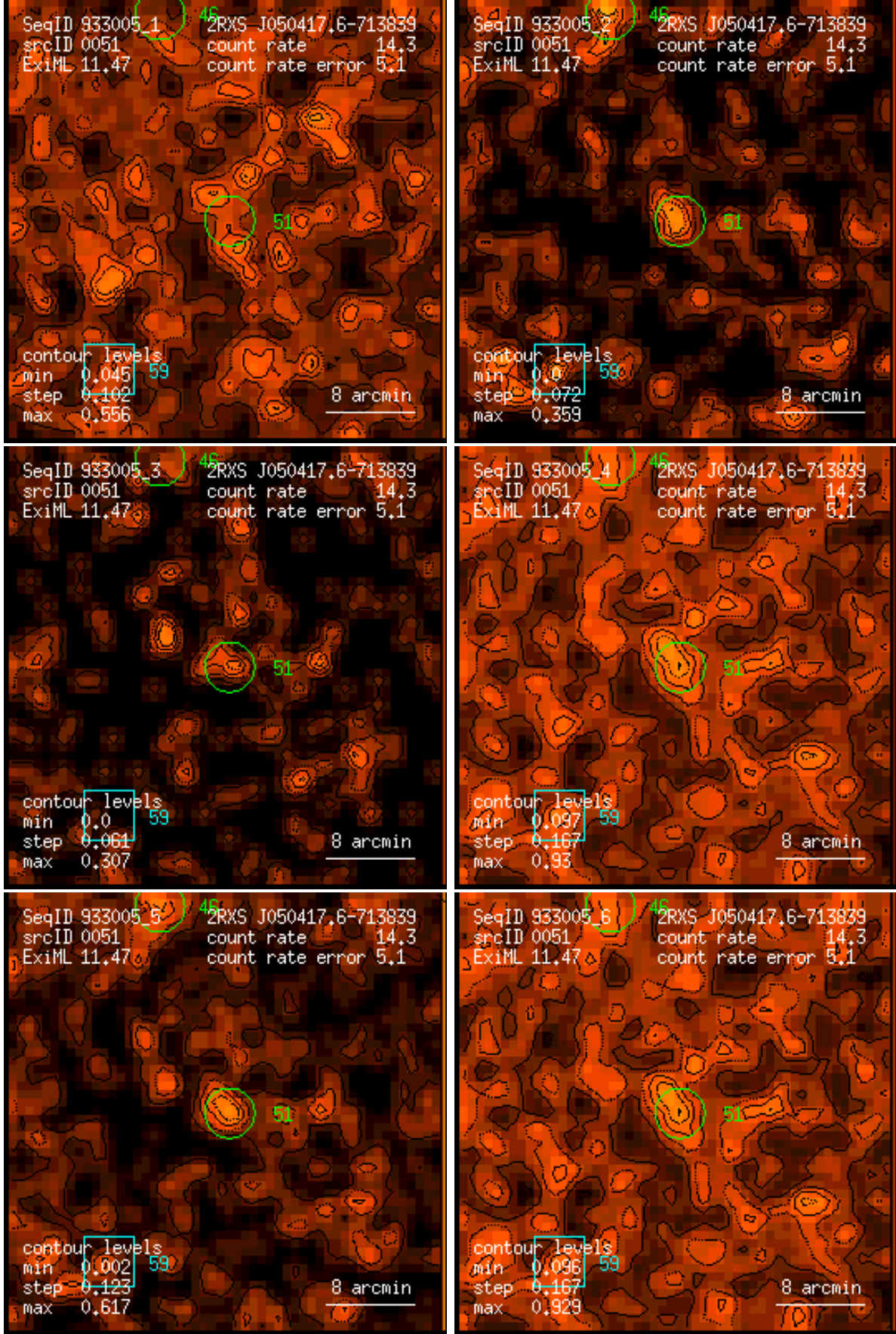
Figure 51: RASS 933005: detection 0051: band rate images, Gaussian filter: (1) PSPC channels 11 – 41, (2) 52 – 90, (3) 91 – 201, (4) 11 – 235, (5) 52 – 201, (6) 11 – 201. Broad band rates in counts/ks. Band rate contour levels in counts/ks/arcmin 2 .
