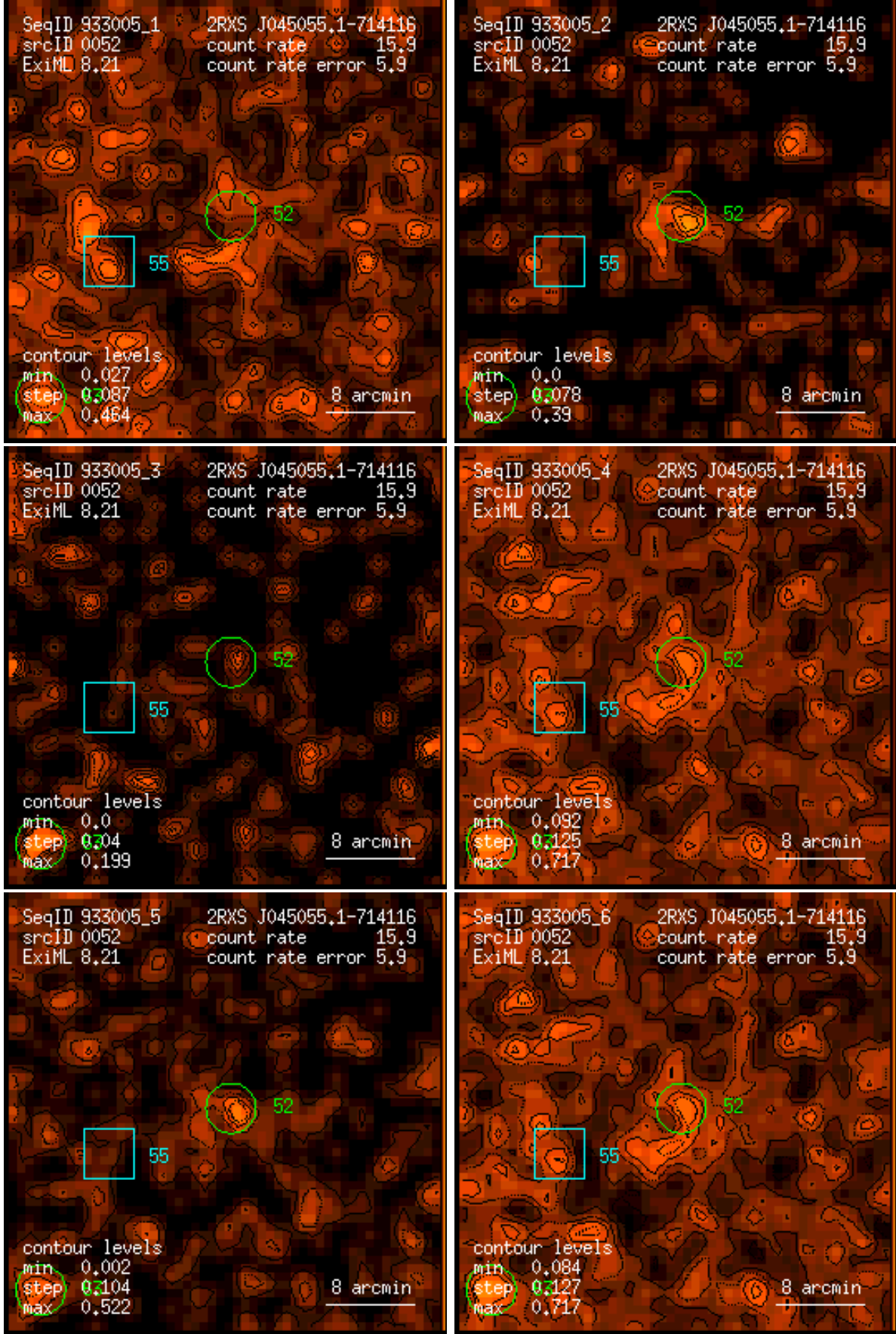
Figure 52: RASS 933005: detection 0052: band rate images, Gaussian filter: (1) PSPC channels 11 – 41, (2) 52 – 90, (3) 91 – 201, (4) 11 – 235, (5) 52 – 201, (6) 11 – 201. Broad band rates in counts/ks. Band rate contour levels in counts/ks/arcmin 2 .
