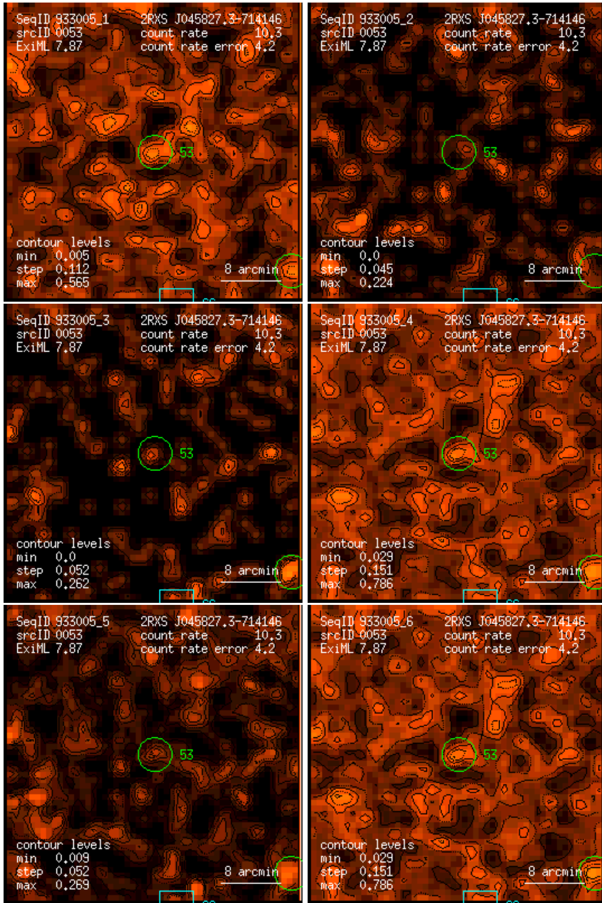
Figure 53: RASS 933005: detection 0053: band rate images, Gaussian filter: (1) PSPC channels 11 – 41, (2) 52 – 90, (3) 91 – 201, (4) 11 – 235, (5) 52 – 201, (6) 11 – 201. Broad band rates in counts/ks. Band rate contour levels in counts/ks/arcmin 2 .
