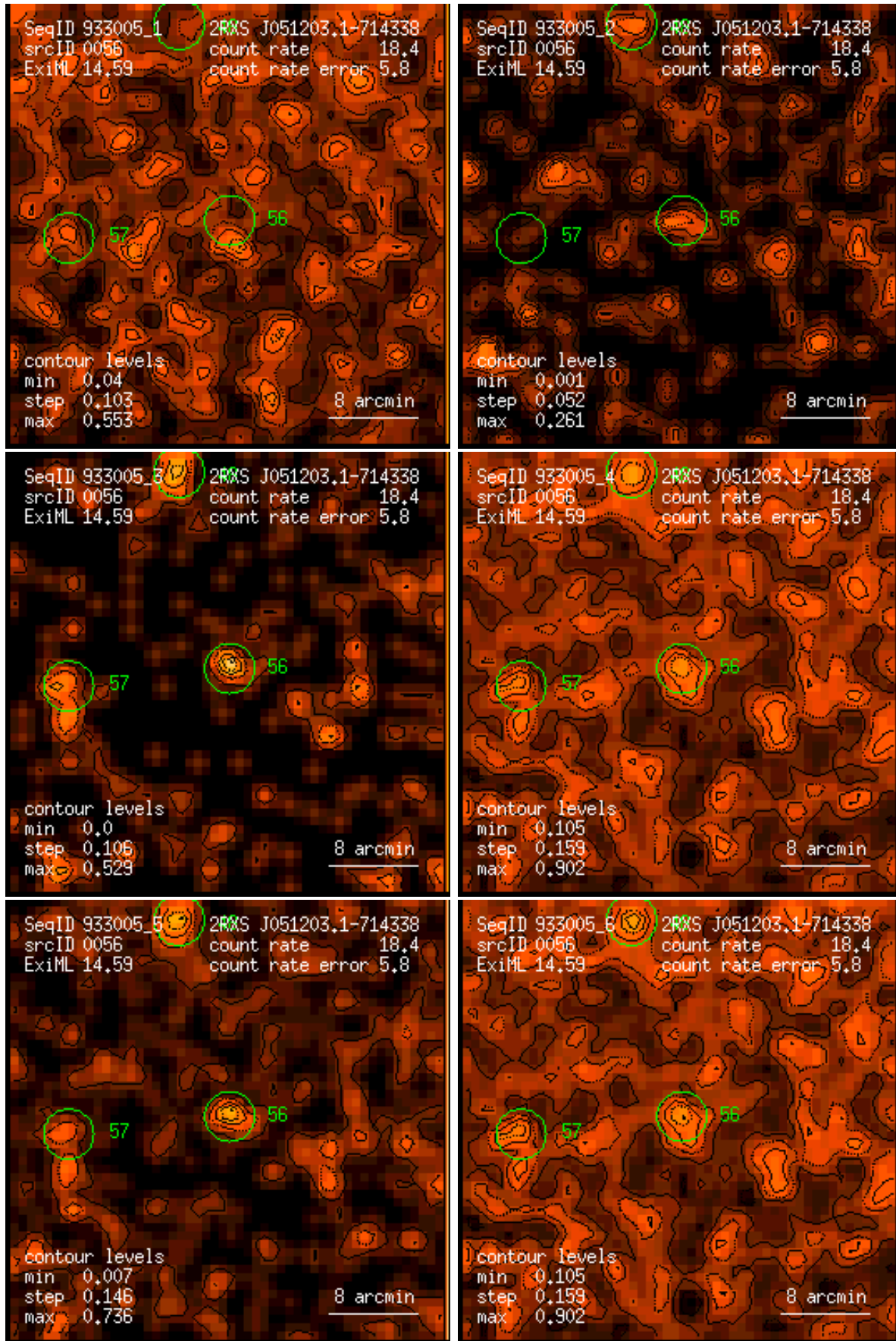
Figure 56: RASS 933005: detection 0056: band rate images, Gaussian filter: (1) PSPC channels 11 – 41, (2) 52 – 90, (3) 91 – 201, (4) 11 – 235, (5) 52 – 201, (6) 11 – 201. Broad band rates in counts/ks. Band rate contour levels in counts/ks/arcmin 2 .
