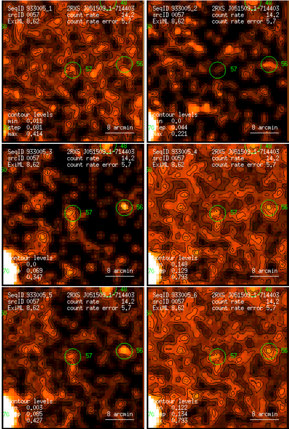
Figure 57: RASS 933005: detection 0057: band rate images, Gaussian filter: (1) PSPC channels 11 – 41, (2) 52 – 90, (3) 91 – 201, (4) 11 – 235, (5) 52 – 201, (6) 11 – 201. Broad band rates in counts/ks. Band rate contour levels in counts/ks/arcmin 2 .
