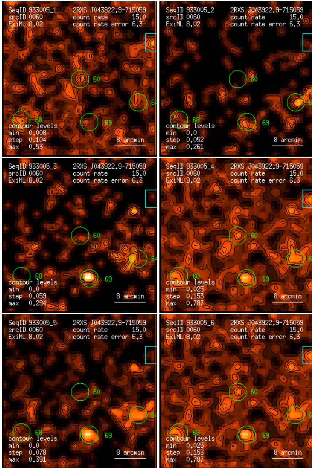
Figure 60: RASS 933005: detection 0060: band rate images, Gaussian filter: (1) PSPC channels 11 – 41, (2) 52 – 90, (3) 91 – 201, (4) 11 – 235, (5) 52 – 201, (6) 11 – 201. Broad band rates in counts/ks. Band rate contour levels in counts/ks/arcmin 2 .
