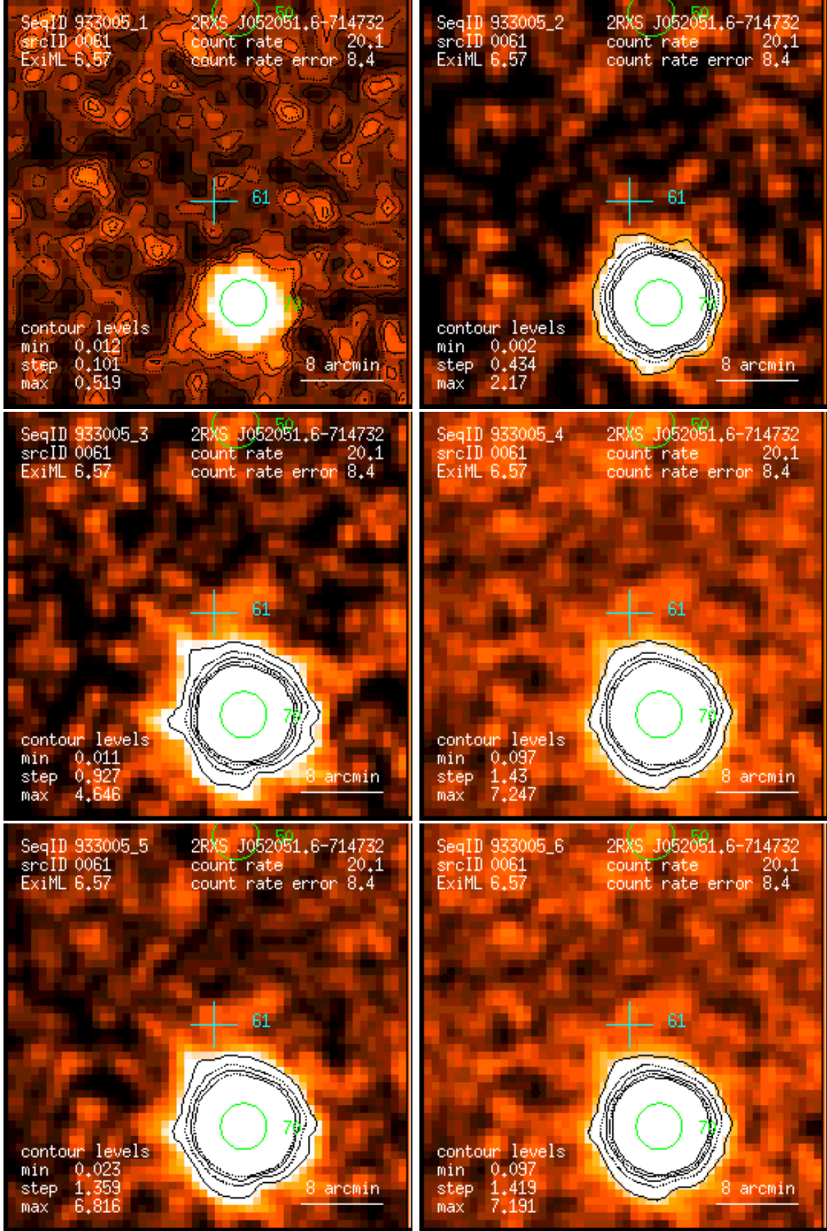
Figure 61: RASS 933005: detection 0061: band rate images, Gaussian filter: (1) PSPC channels 11 – 41, (2) 52 – 90, (3) 91 – 201, (4) 11 – 235, (5) 52 – 201, (6) 11 – 201. Broad band rates in counts/ks. Band rate contour levels in counts/ks/arcmin 2 .
