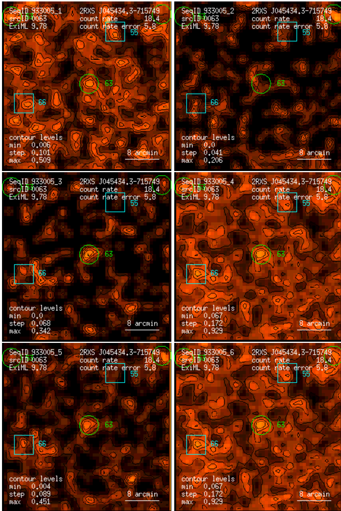
Figure 63: RASS 933005: detection 0063: band rate images, Gaussian filter: (1) PSPC channels 11 – 41, (2) 52 – 90, (3) 91 – 201, (4) 11 – 235, (5) 52 – 201, (6) 11 – 201. Broad band rates in counts/ks. Band rate contour levels in counts/ks/arcmin 2 .
