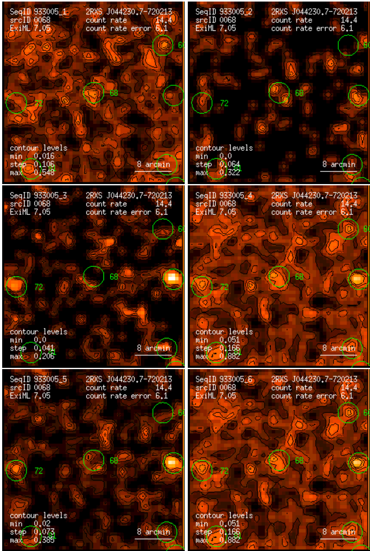
Figure 68: RASS 933005: detection 0068: band rate images, Gaussian filter: (1) PSPC channels 11 – 41, (2) 52 – 90, (3) 91 – 201, (4) 11 – 235, (5) 52 – 201, (6) 11 – 201. Broad band rates in counts/ks. Band rate contour levels in counts/ks/arcmin 2 .
