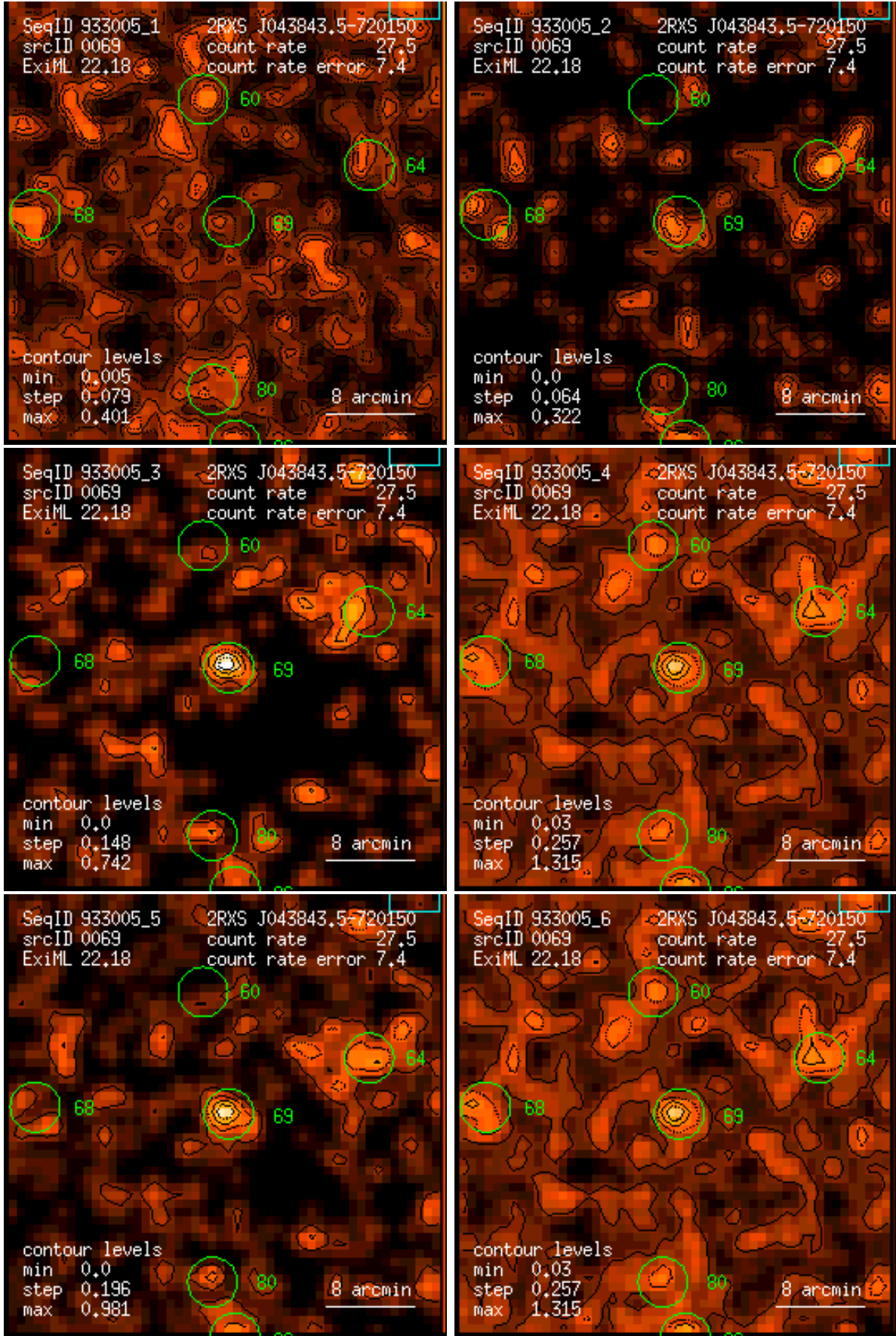
Figure 69: RASS 933005: detection 0069: band rate images, Gaussian filter: (1) PSPC channels 11 – 41, (2) 52 – 90, (3) 91 – 201, (4) 11 – 235, (5) 52 – 201, (6) 11 – 201. Broad band rates in counts/ks. Band rate contour levels in counts/ks/arcmin 2 .
