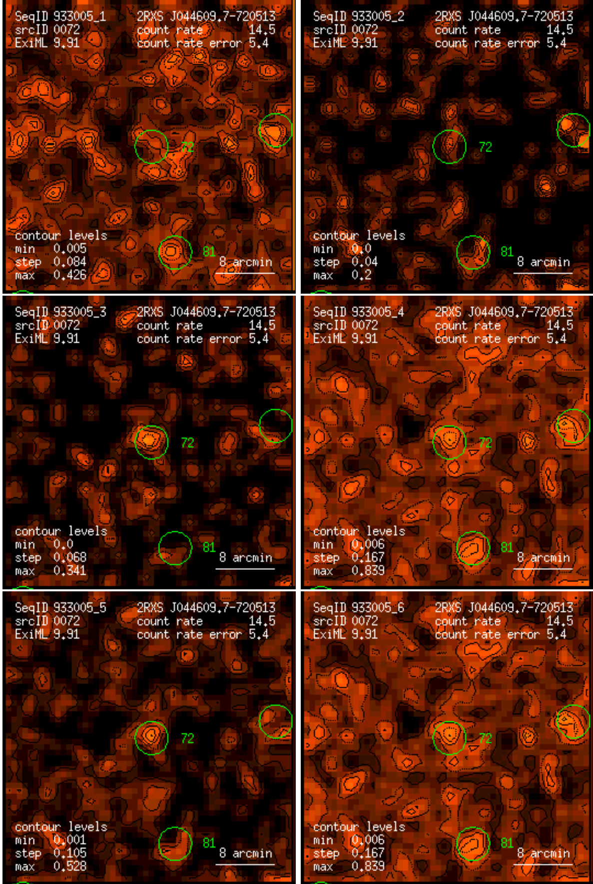
Figure 72: RASS 933005: detection 0072: band rate images, Gaussian filter: (1) PSPC channels 11 – 41, (2) 52 – 90, (3) 91 – 201, (4) 11 – 235, (5) 52 – 201, (6) 11 – 201. Broad band rates in counts/ks. Band rate contour levels in counts/ks/arcmin 2 .
