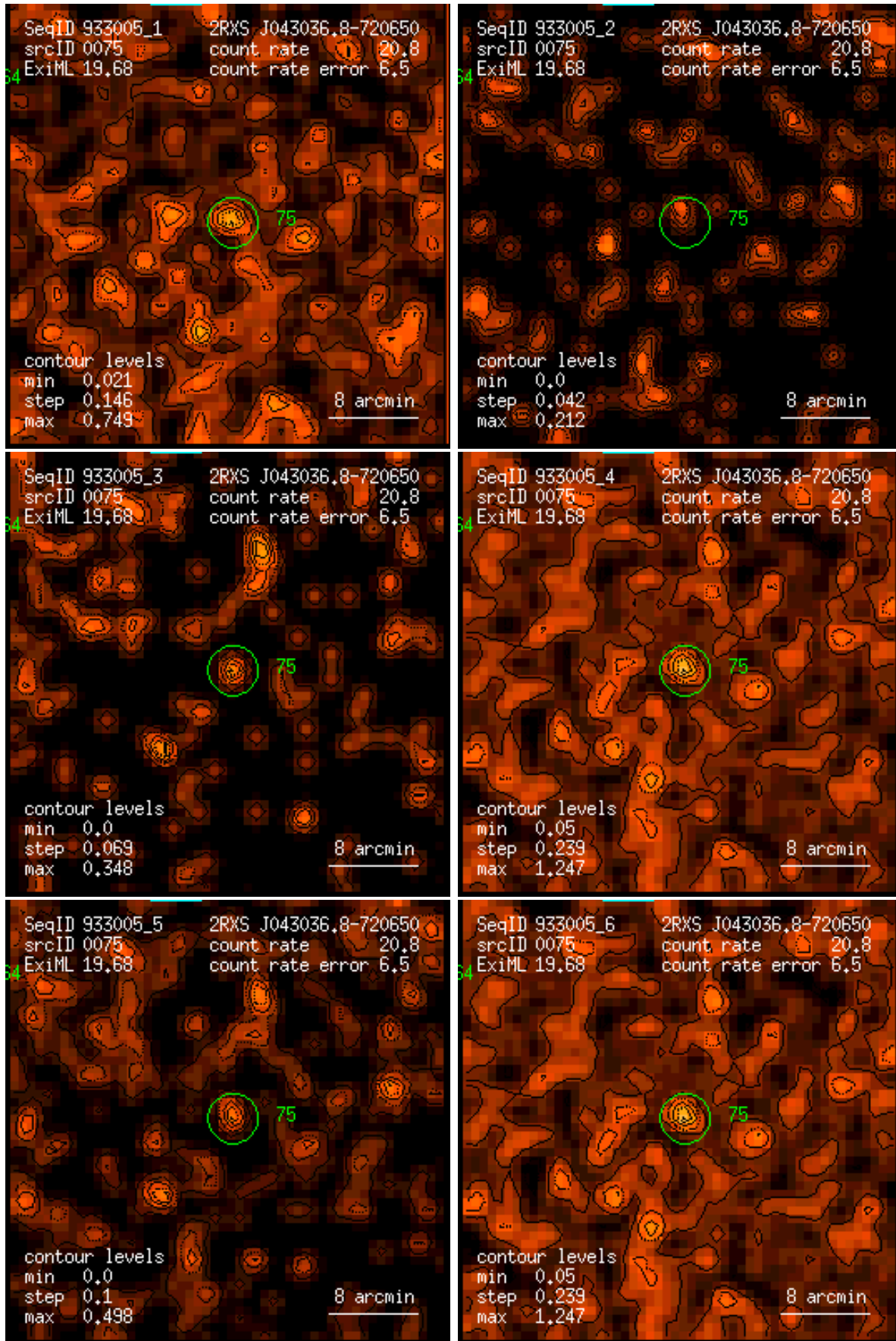
Figure 75: RASS 933005: detection 0075: band rate images, Gaussian filter: (1) PSPC channels 11 – 41, (2) 52 – 90, (3) 91 – 201, (4) 11 – 235, (5) 52 – 201, (6) 11 – 201. Broad band rates in counts/ks. Band rate contour levels in counts/ks/arcmin 2 .
