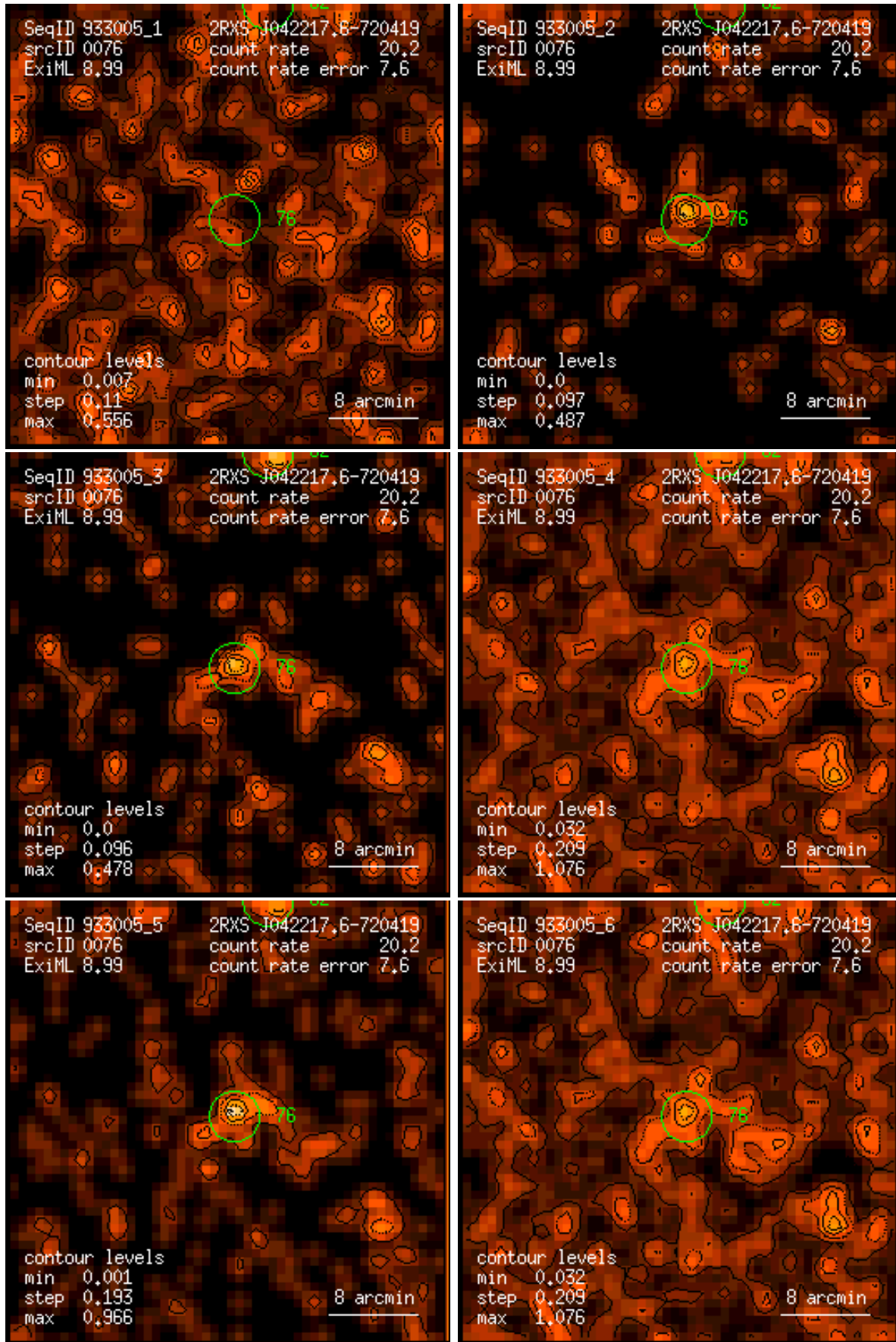
Figure 76: RASS 933005: detection 0076: band rate images, Gaussian filter: (1) PSPC channels 11 – 41, (2) 52 – 90, (3) 91 – 201, (4) 11 – 235, (5) 52 – 201, (6) 11 – 201. Broad band rates in counts/ks. Band rate contour levels in counts/ks/arcmin 2 .
