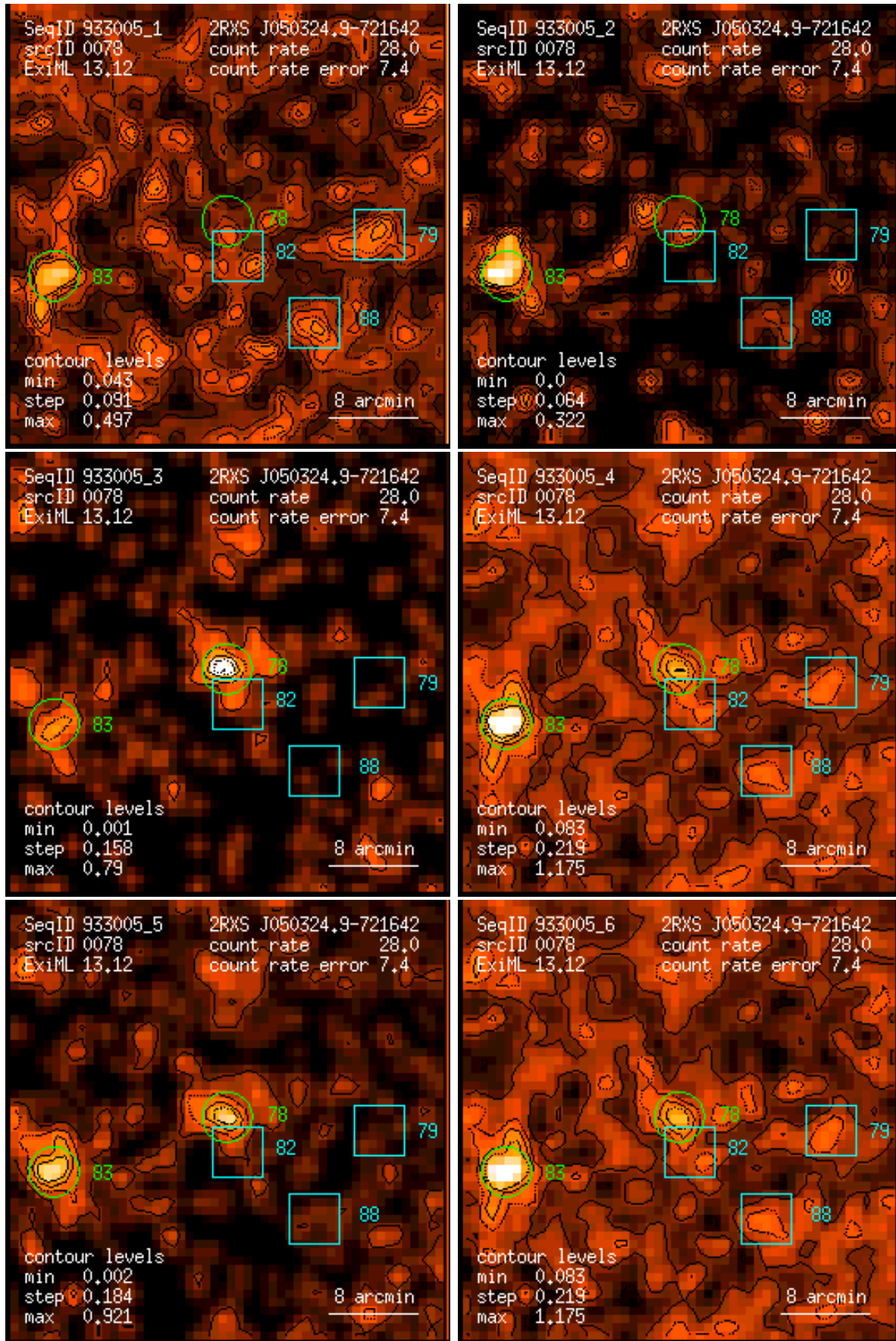
Figure 78: RASS 933005: detection 0078: band rate images, Gaussian filter: (1) PSPC channels 11 – 41, (2) 52 – 90, (3) 91 – 201, (4) 11 – 235, (5) 52 – 201, (6) 11 – 201. Broad band rates in counts/ks. Band rate contour levels in counts/ks/arcmin 2 .
