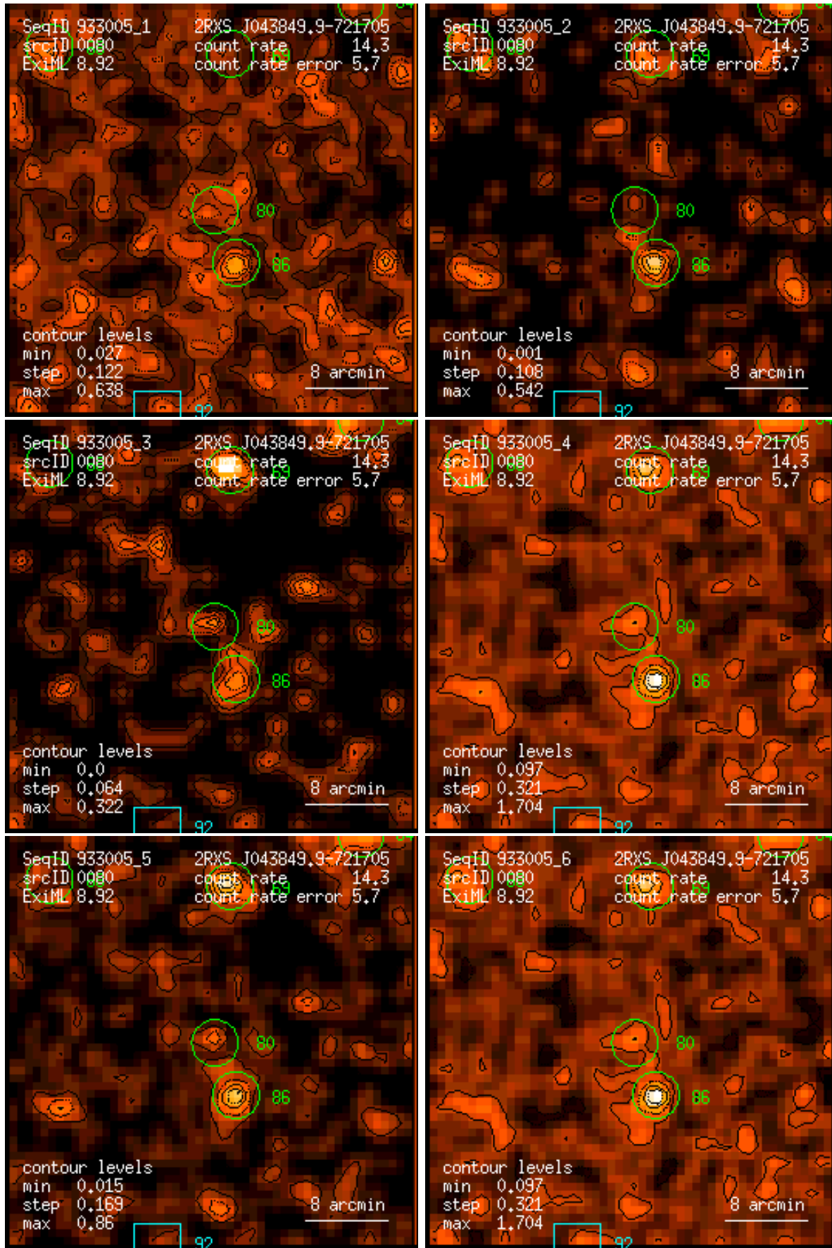
Figure 80: RASS 933005: detection 0080: band rate images, Gaussian filter: (1) PSPC channels 11 – 41, (2) 52 – 90, (3) 91 – 201, (4) 11 – 235, (5) 52 – 201, (6) 11 – 201. Broad band rates in counts/ks. Band rate contour levels in counts/ks/arcmin 2 .
