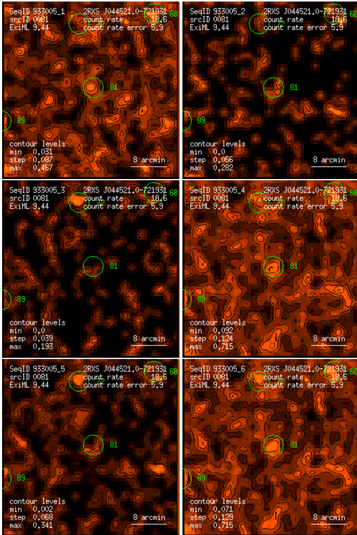
Figure 81: RASS 933005: detection 0081: band rate images, Gaussian filter: (1) PSPC channels 11 – 41, (2) 52 – 90, (3) 91 – 201, (4) 11 – 235, (5) 52 – 201, (6) 11 – 201. Broad band rates in counts/ks. Band rate contour levels in counts/ks/arcmin 2 .
