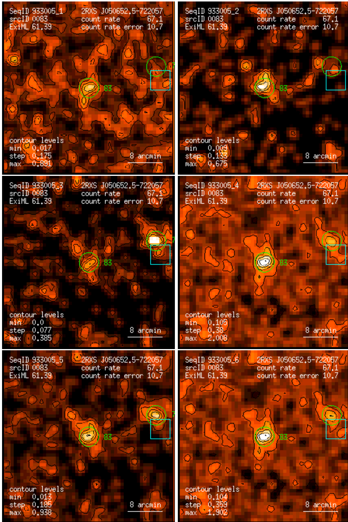
Figure 83: RASS 933005: detection 0083: band rate images, Gaussian filter: (1) PSPC channels 11 – 41, (2) 52 – 90, (3) 91 – 201, (4) 11 – 235, (5) 52 – 201, (6) 11 – 201. Broad band rates in counts/ks. Band rate contour levels in counts/ks/arcmin 2 .
