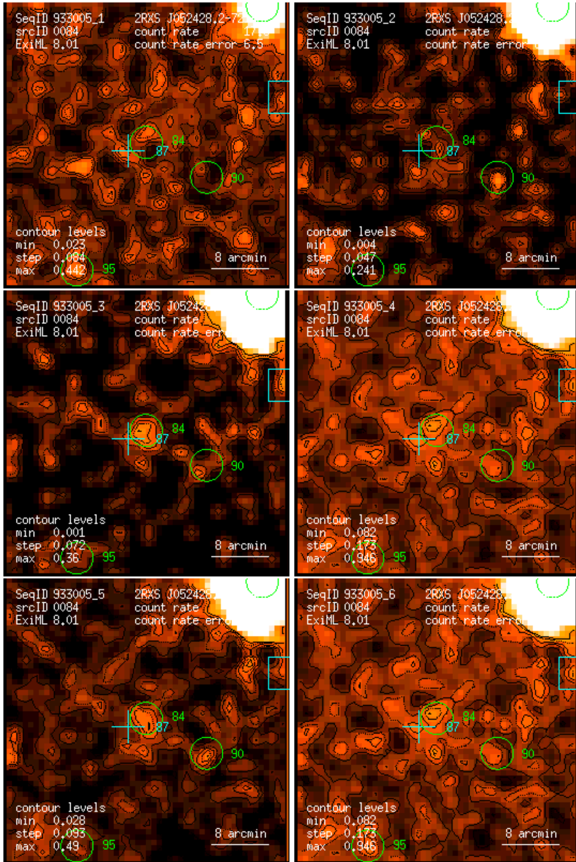
Figure 84: RASS 933005: detection 0084: band rate images, Gaussian filter: (1) PSPC channels 11 – 41, (2) 52 – 90, (3) 91 – 201, (4) 11 – 235, (5) 52 – 201, (6) 11 – 201. Broad band rates in counts/ks. Band rate contour levels in counts/ks/arcmin 2 .
