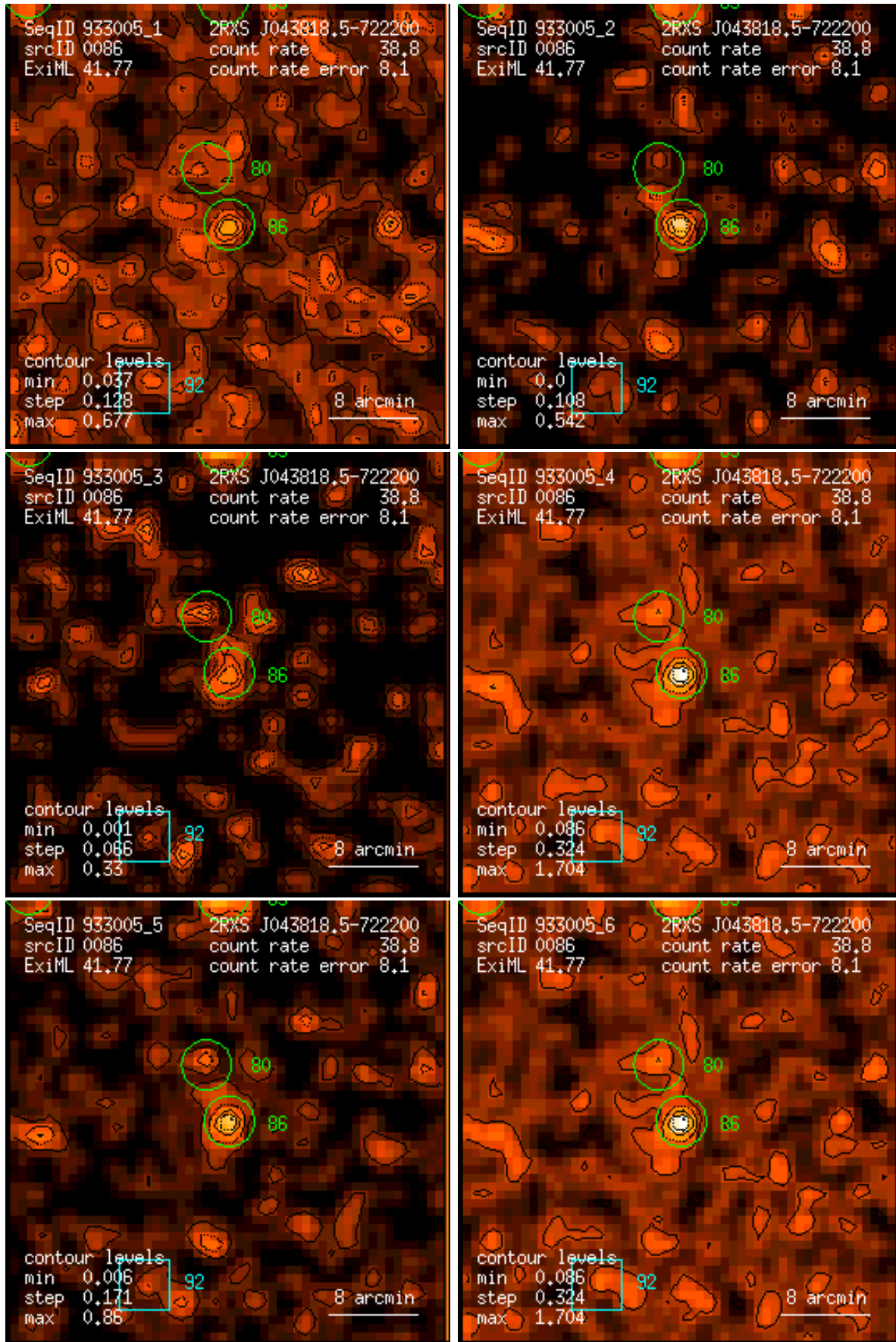
Figure 86: RASS 933005: detection 0086: band rate images, Gaussian filter: (1) PSPC channels 11 – 41, (2) 52 – 90, (3) 91 – 201, (4) 11 – 235, (5) 52 – 201, (6) 11 – 201. Broad band rates in counts/ks. Band rate contour levels in counts/ks/arcmin 2 .
