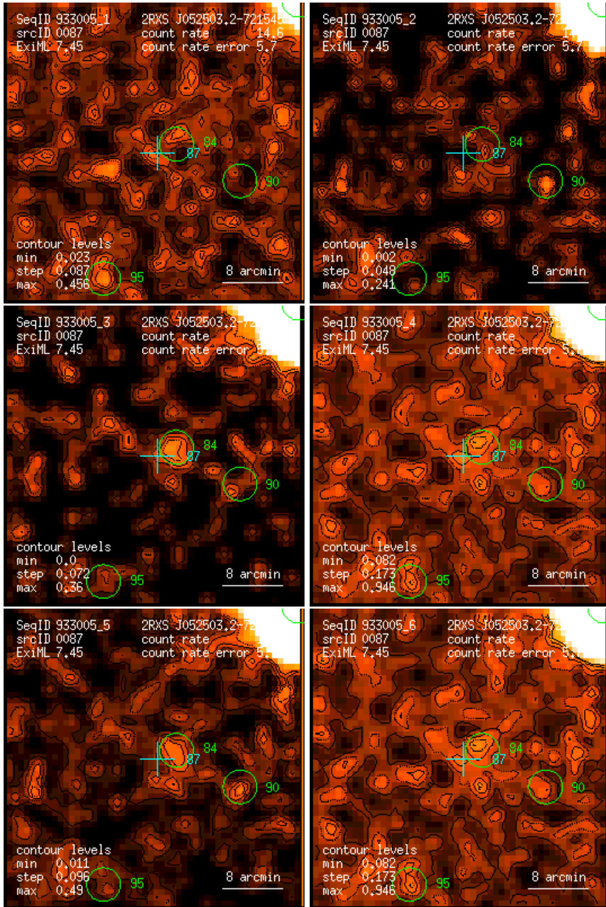
Figure 87: RASS 933005: detection 0087: band rate images, Gaussian filter: (1) PSPC channels 11 – 41, (2) 52 – 90, (3) 91 – 201, (4) 11 – 235, (5) 52 – 201, (6) 11 – 201. Broad band rates in counts/ks. Band rate contour levels in counts/ks/arcmin 2 .
