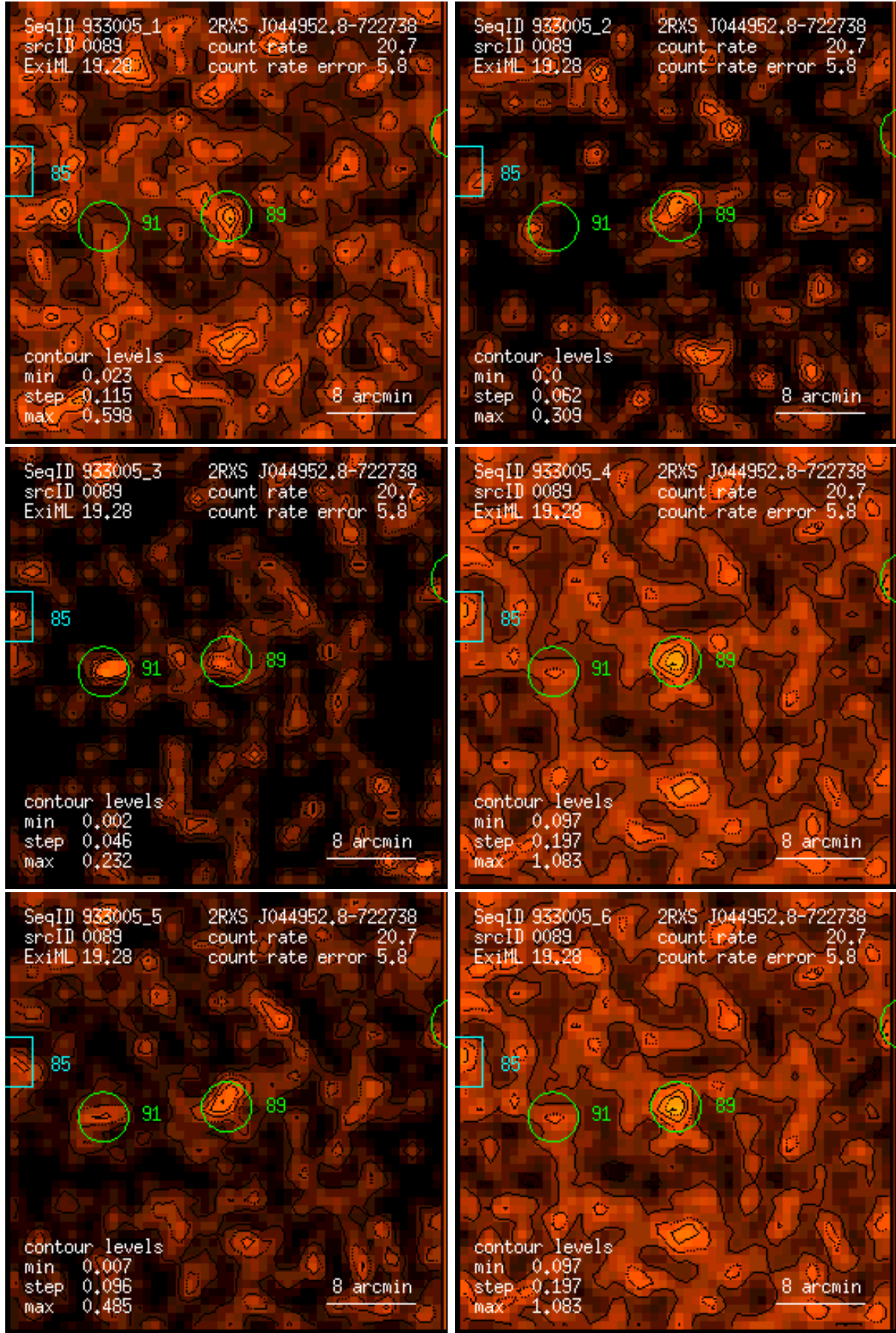
Figure 89: RASS 933005: detection 0089: band rate images, Gaussian filter: (1) PSPC channels 11 – 41, (2) 52 – 90, (3) 91 – 201, (4) 11 – 235, (5) 52 – 201, (6) 11 – 201. Broad band rates in counts/ks. Band rate contour levels in counts/ks/arcmin 2 .
