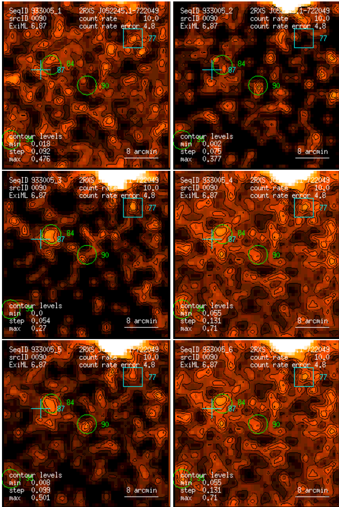
Figure 90: RASS 933005: detection 0090: band rate images, Gaussian filter: (1) PSPC channels 11 – 41, (2) 52 – 90, (3) 91 – 201, (4) 11 – 235, (5) 52 – 201, (6) 11 – 201. Broad band rates in counts/ks. Band rate contour levels in counts/ks/arcmin 2 .
